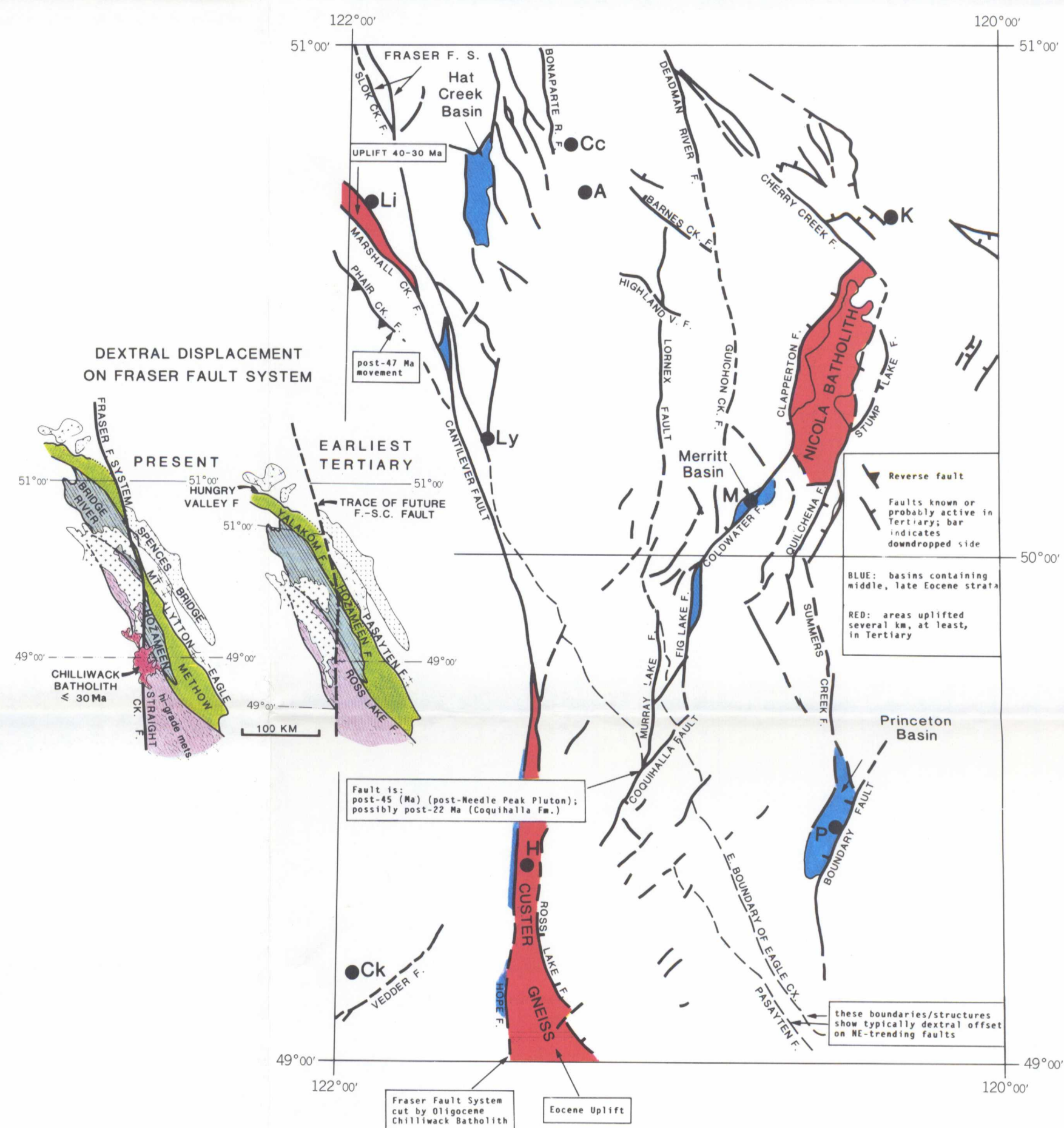
Figure D: Tertiary structural elements in Hope and Ashcroft map areas
