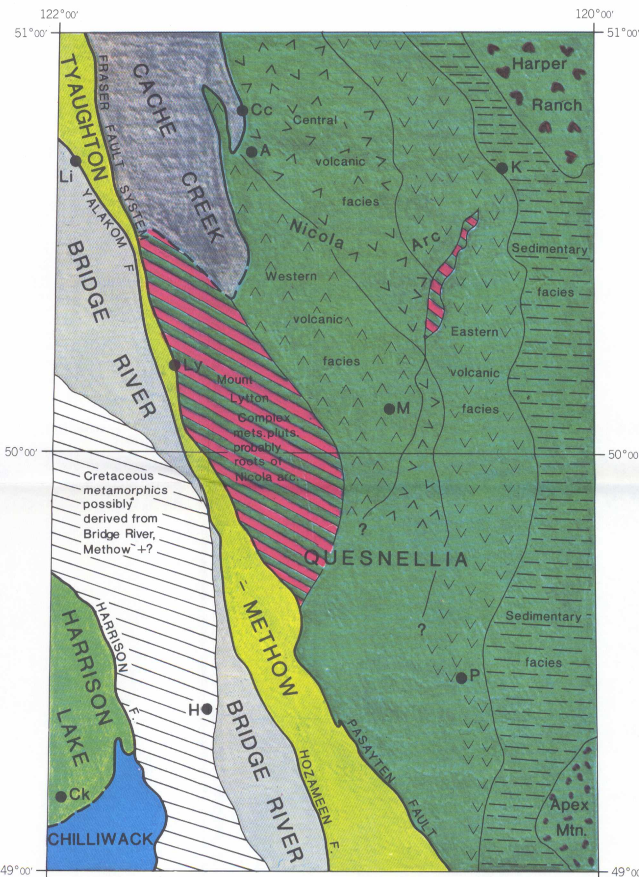
Figure A: Distribution of terranes and major, terrane-bounding faults in Hope and Ashcroft map areas. Facies within the Upper Triassic Nicola Group, which characterizes Quesnellia, are shown. Principal settlements: A, Ashcroft; H, Hope; K, Kamloops; Li, Lillooet; Ly, Lytton; M, Merritt; P, Princeton; Cc, Cache Creek; Ck, Chilliwack
