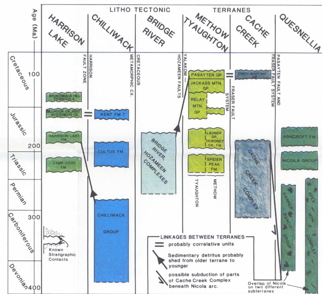
Figure B: Rock units of terranes in Hope and Ashcroft map areas, showing known and possible linkages between terranes
