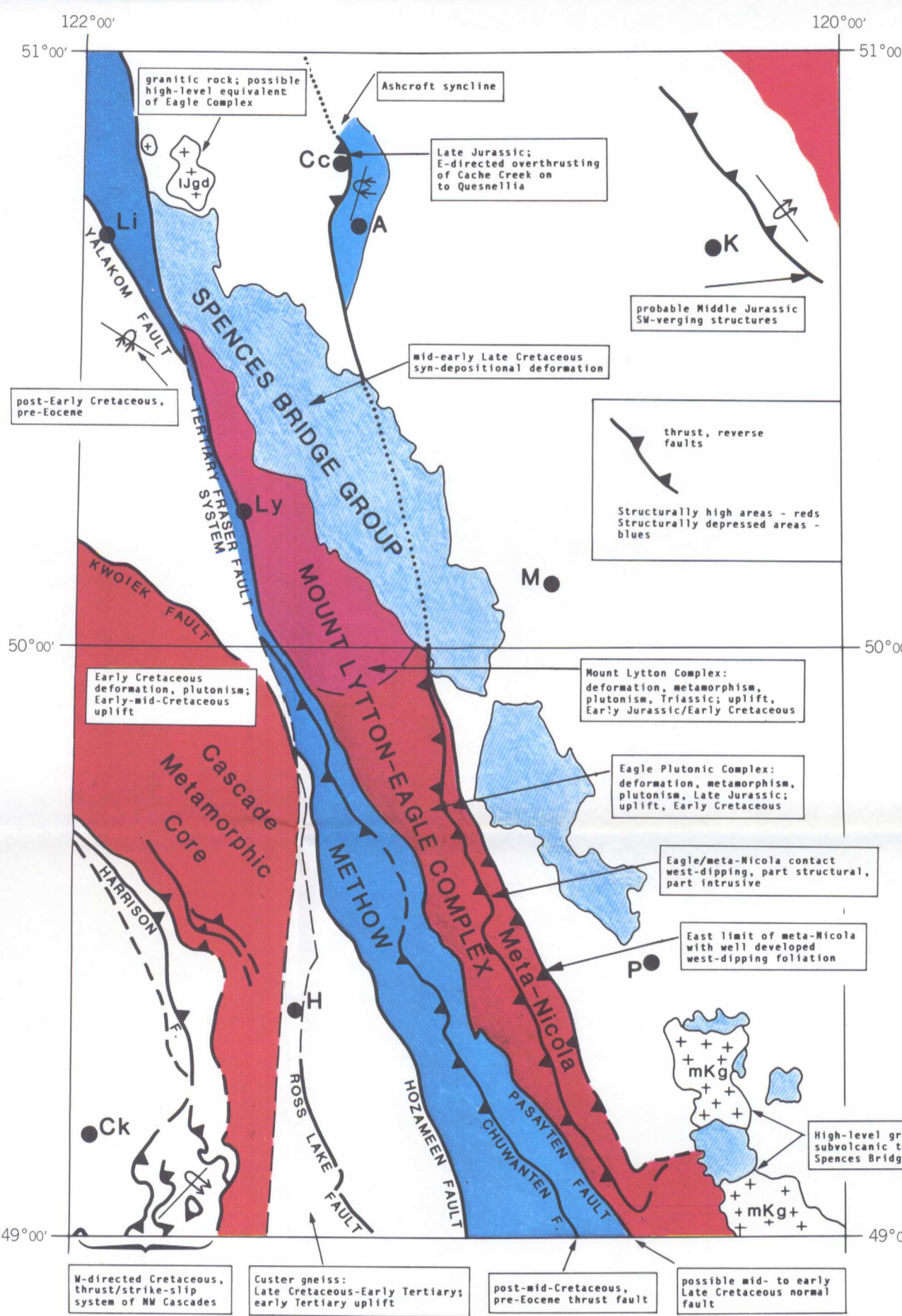
Figure C: Jurassic and Cretaceous structural elements in Hope and Ashcroft map areas
