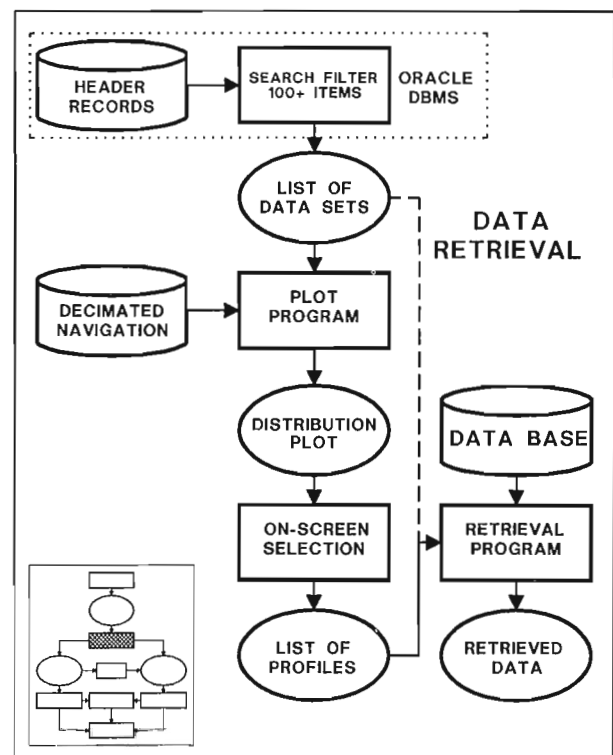
Figure 3. Index and retrieval procedures: header records and decimated navigation are stored on line and are queried interactively (depending on the user's needs, the production of a track plot from the decimated navigation is an optional step that can be bypassed); the output is a set of batch commands for extracting selected data sets from the main data base, which is stored off line.
