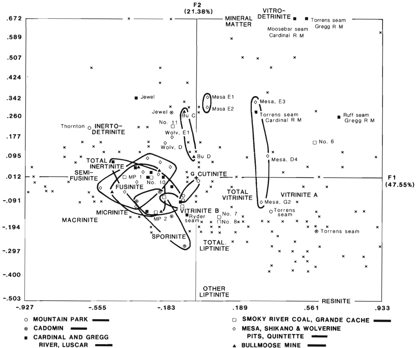
Figure 6. Projection plan from correspondence analysis of a data set containing data from coals formed during the Early Cretaceous. The positions of the different macerals relative to the different localities help toward the elaboration of a geological model. (After Kalkreuth et al., 1989.)
