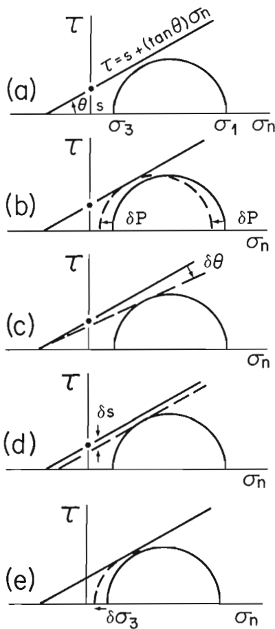
Figure 5. Trigger mechanisms for fault on verge of failure: Part (a) shows Coulomb-Mohr failure diagram for fault with low cohesive strength ( s ), coefficient of friction ( \tan \theta ), maximum ( \sigma_1 ), minimum ( \sigma_3 ), and normal ( \sigma_n ) stress. Part (b) shows effect of increase in pore pressure ( \delta P ). Part (c) shows decrease in angle of friction ( \delta \theta ) as consequence of fault gouge. Part (d) shows decrease in cohesive strength ( \delta s ) of asperity that binds fault. Part (e) shows decrease in minimum principal stress ( \delta \sigma_3 ) for thrust-fault environment as consequence of mine excavation.
