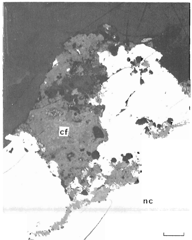
Figure 4. Coffinite (cf) surrounding and replacing nickeline (nc). Collins Bay "B" deposit. Photomicrograph, reflected light. Scale bar is equal to 100 \mu m.
