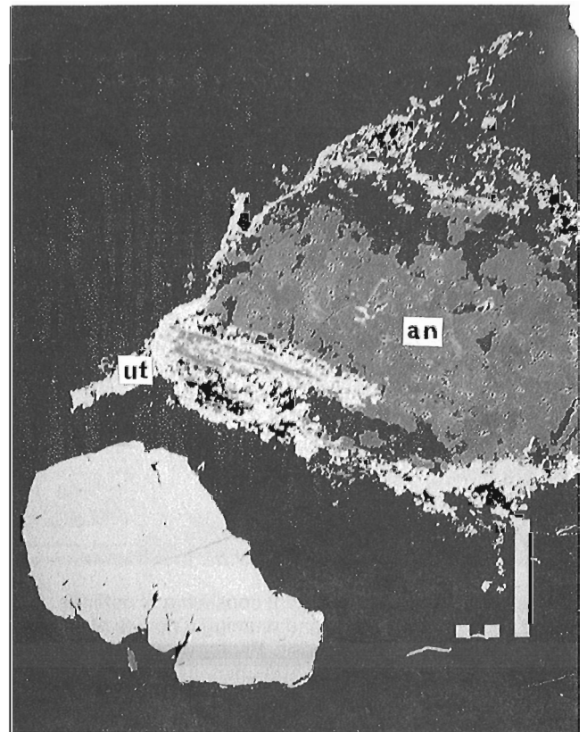
Figure 8. A U-Ti-(Si) phase ("brannerite") (ut) partly replacing rim of an anatase (an) grain. Spine Road occurrence, Elliot Lake. Backscattered electron photograph. Scale bar is equal to 100 \mu\text{m} .
