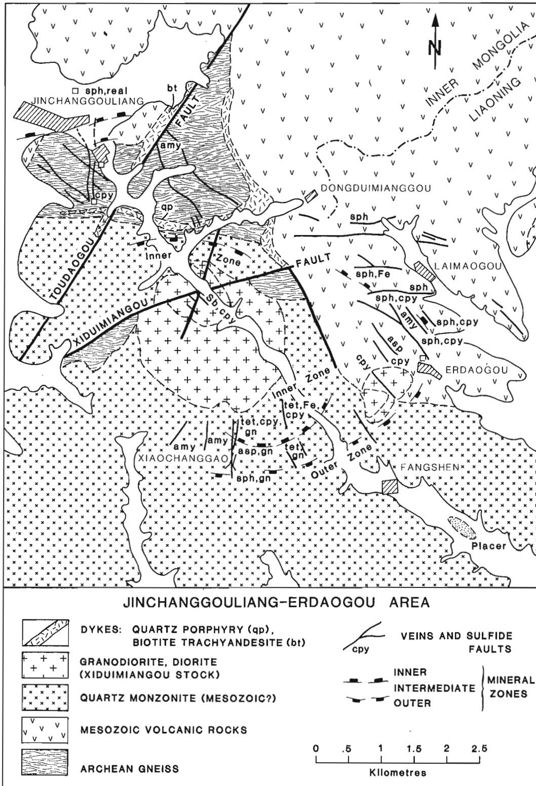
Figure 4. Map of the geology and gold veins in the Jinchanggouliang-Erdaogou area showing the boundaries of mineral zones. Mineral abbreviations are amy (amethyst), Fl (fluorite), tet (tetrahydrate), cpy (chalcopyrite), asp (arsenopyrite), sph (sphalerite), gn (galena), sb (stibnite), and real (realgar).
