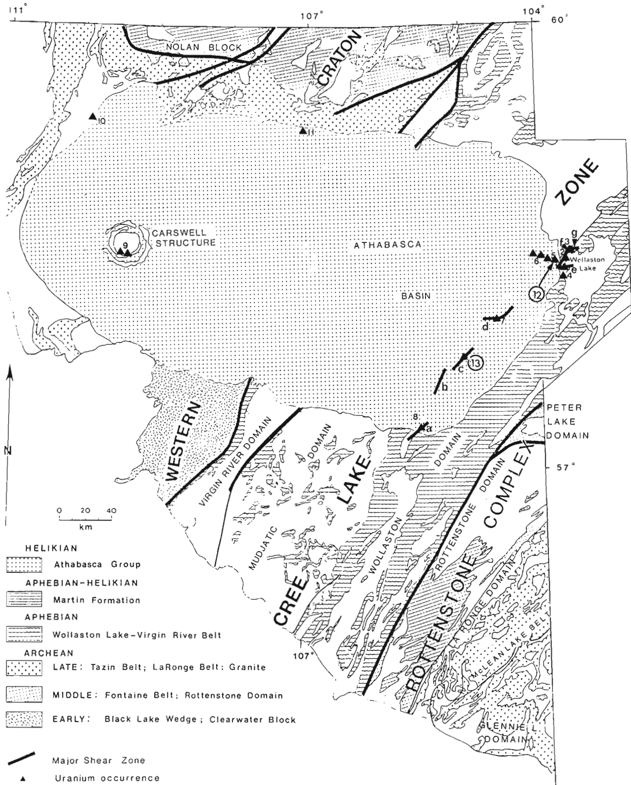
Figure 1. Selected uranium occurrences and structural trends controlling uranium mineralization in the Athabasca Basin region. Occurrences: 1 = Rabbit Lake; 2 = Collins Bay "A", "B" and "D"; 3 = Eagle Point; 4 = Raven and Horseshoe; 5 = McClean; 6 = Midwest and Dawn Lake; 7 = Cigar Lake; 8 = Key Lake; 9 = Cluff "D", Claude, OP, Dominique-Peter, Dominique-Janine, and South Dominique-Janine; 10 = Maurice Bay; 11 = Fond-du-Lac; 12 (circled) = Sue zone; 13 (circled) = P2N zone. Structures: a = Key Lake Fault; b = Hughes-Mann Lake Fault; c = P2 Fault; d = Cigar Lake Shear Zone; e = Rabbit Lake Fault; f = Collins Bay Fault Zone; g = Eagle Point Fault. Base map after Lewry and Sibbald (1979).
