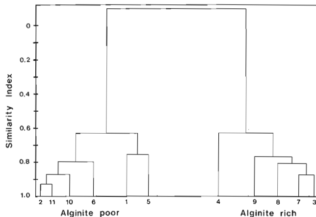
Figure 3. Dendograph showing the similarity indexes between the oil shales from Grinnell Peninsula, Emma Fjord Formation, Arctic Archipelago, based on a comparison of all variables — chemical, petrographic, and boron content. (After Goodarzi et al., 1987.)
