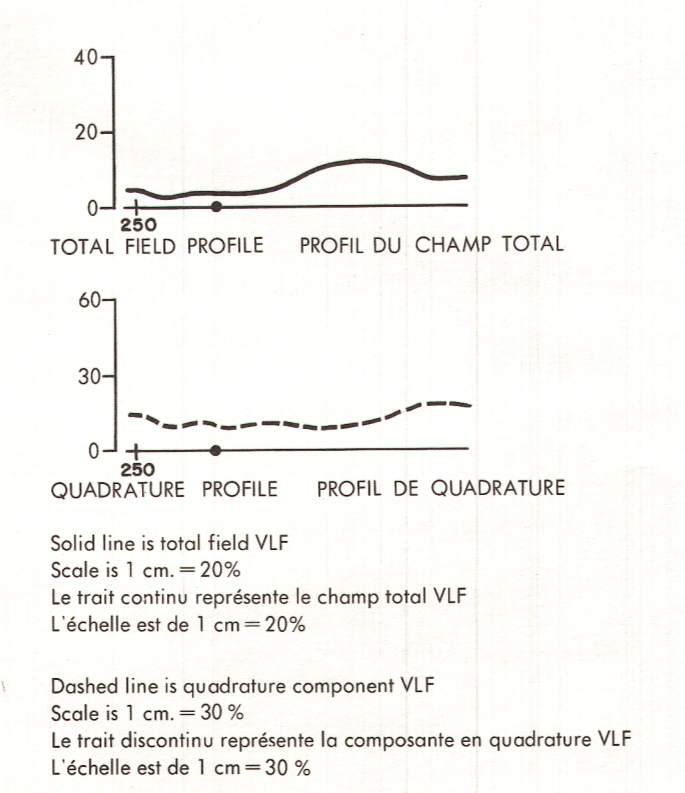
TOTEM VLF EM PROFILES FOR ORTHOGONAL STATION PROFILS DE TOTEM EM VLF POUR LA STATION ORTHOGONALE
