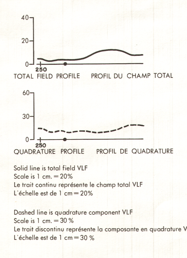
TOTEM VLF EM PROFILES FOR ORTHOGONAL STATION PROFILS DE TOTEM EM VLF POUR LA STATION ORTHOGONALE
