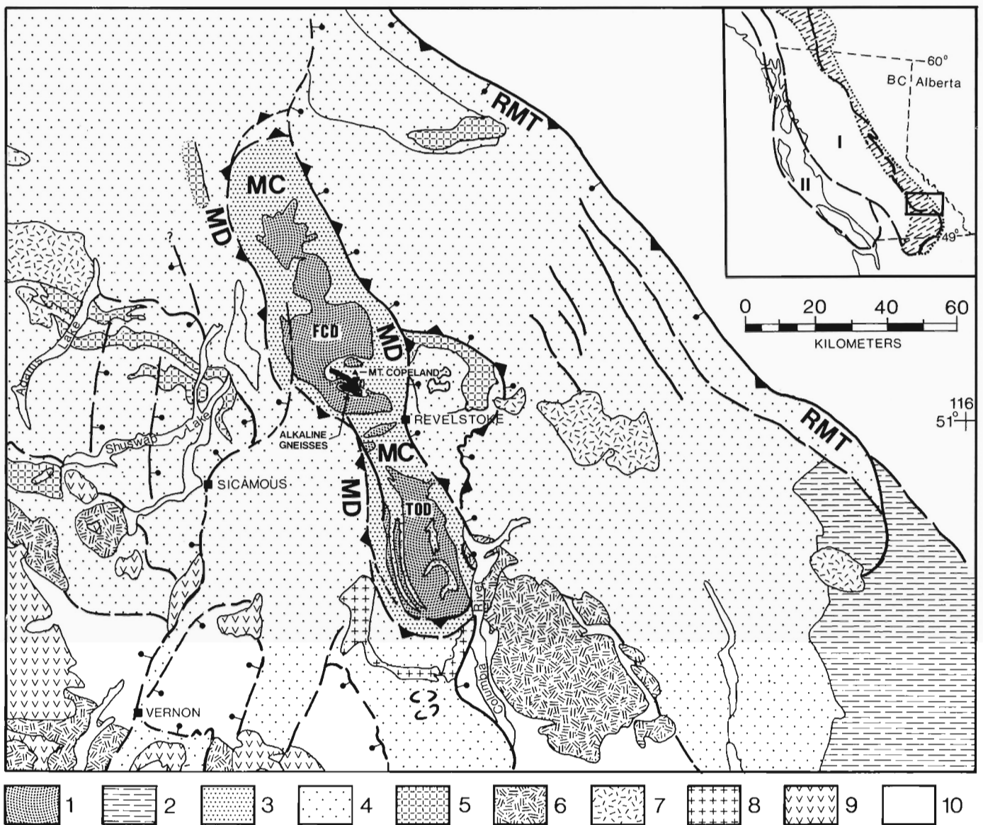
Figure 1. Tectonic map of southeastern British Columbia, modified after Hoy and Brown (1980), Journey and Brown (1986), and Parrish et al. (1988). Faults marked in heavy lines are thrust faults (barbs), and normal faults (dots) with notation on the hangingwalls, and include the Monashee décollement (MD) and the Rocky Mountain Trench (RMT). On the eastern side of the Monashee Complex, the Monashee décollement is coincident with the Columbia River normal fault (identified by normal fault symbols). Map units are (1) Aphebian core gneiss of the Monashee Complex, (2) Mid-Late Proterozoic Belt-Purcell Supergroup, (3) Mantling gneiss of the Monashee Complex, (4) Late Proterozoic Windermere Supergroup, Paleozoic metasedimentary rocks of North American affinity and minor orthogneiss of uncertain age (Selkirk allochthon of Brown and Read, 1983), (5) Paleozoic granitic rocks, (6) Middle Jurassic granitic rocks, (7) Mid-Late Cretaceous granitic rocks, (8) Early-Middle Eocene Ladybird granitic rocks, (9) Miocene-Pliocene basalt, Middle Eocene volcanic and sedimentary rocks, (10) Late Paleozoic-Early Mesozoic allochthonous terrane, and Paleozoic allochthonous ultramafic rocks. FCD, Frenchman Cap dome; TOD, Thor-Odin dome. Inset map outlines the region's location in British Columbia with respect to the Omineca Belt (dashed), and allochthonous terranes I and II (outlined in heavy dashes) of Monger et al. (1982).
