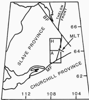
Figure 1. Location of the Moraine Lake transect. H, Healey Lake map sheet; A, Artillery Lake map sheet; BF, Bathurst Fault; MF, MacDonal Fault; MLT, Moraine Lake Transect.
