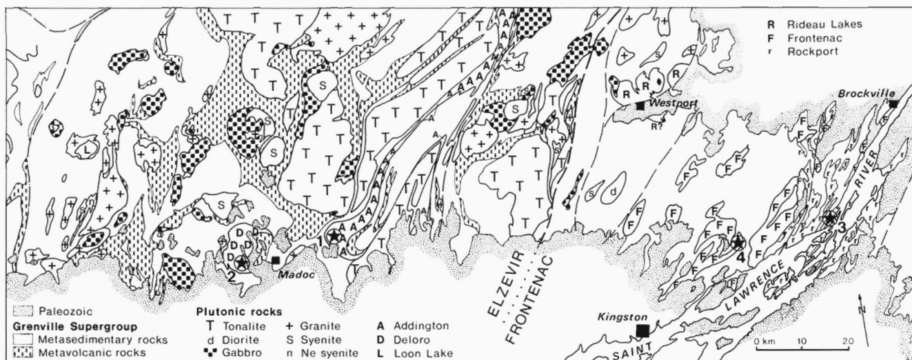
Figure 1. Generalized geology of parts of Elzivir and Frontenac terranes, Central Metasedimentary Belt; their boundary is placed at the easter limit of metavolcanic rocks and tonalitic plutons. Circles stars mark sample locations, numbered as in text and Figures 2 and 3.
