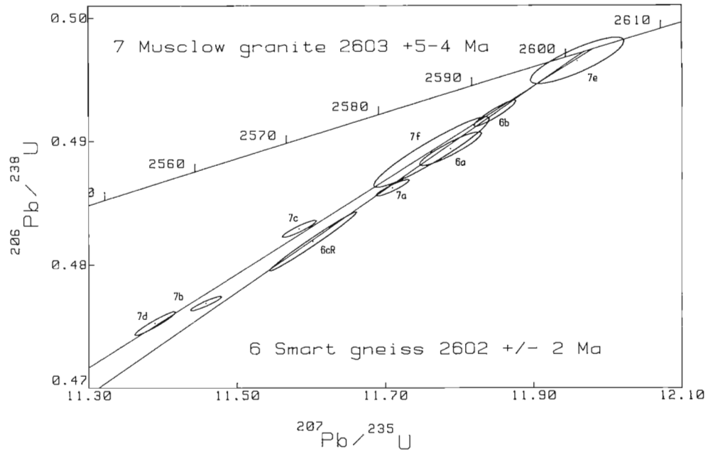
Figure 3. Isotope ratio plot for zircons from 6) Smart gneiss and 7) Musclow granite. Numbers and letters identifying data points correspond to those of Table 1.
