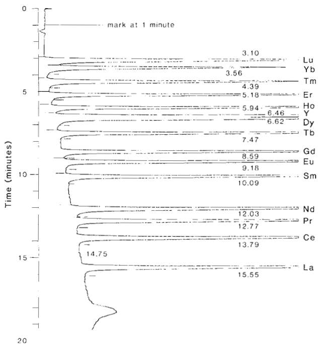
Figure 7: HPLC chromatogram of a 100 microlitre injection of a REE+Y standard (1 microgram each/ml). A gradient elution ranging from 0.05 to 0.40 M HIBA was used with C_8SO_3^- (0.01 M) in the mobile phase to dynamically modify the column. Note the sharp well resolved peaks except for Y which interferes with Dy. The rising baseline is due to the increasing concentration of HIBA.
