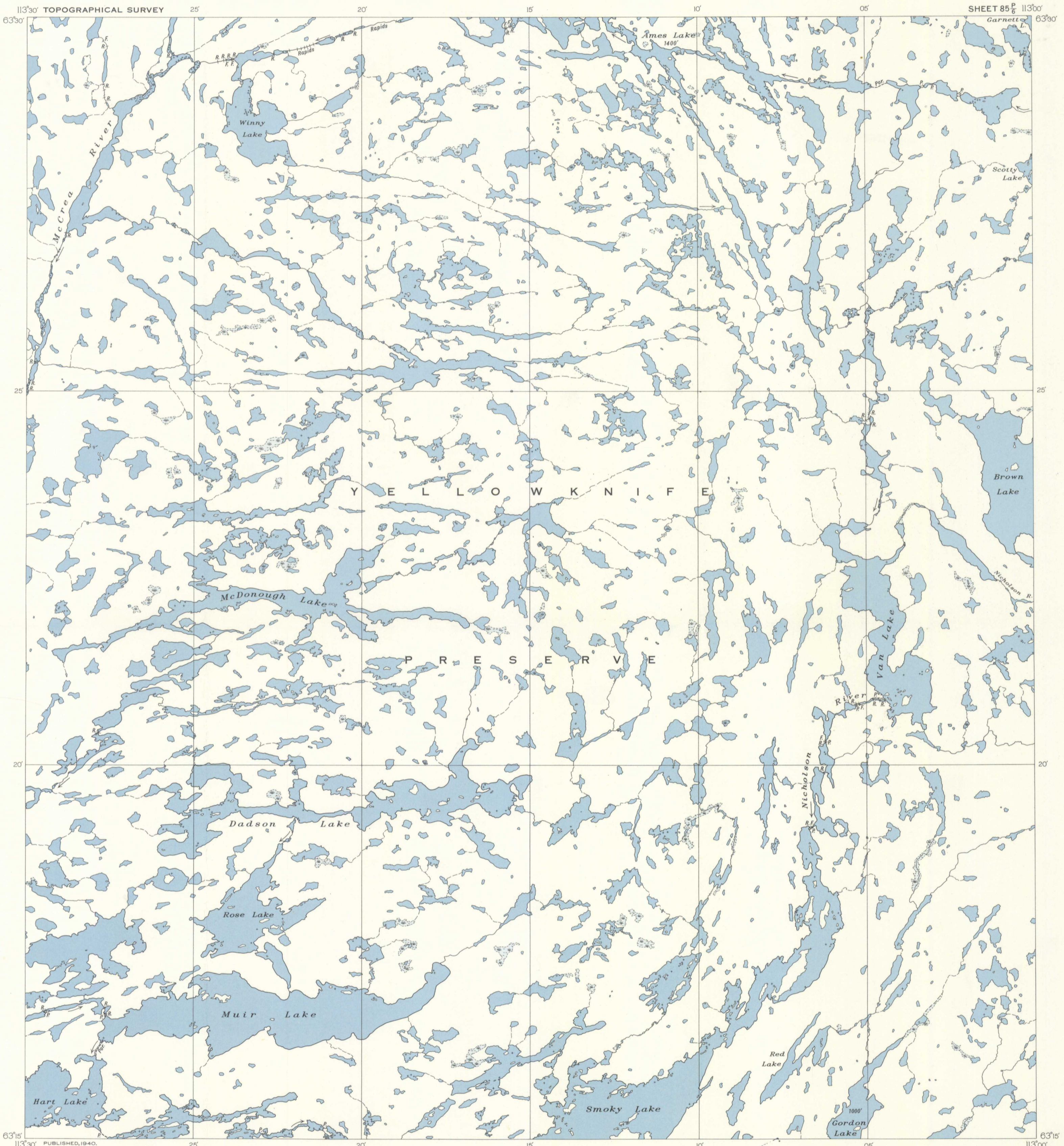
MAP 598A MUIR LAKE DISTRICT OF MACKENZIE NORTHWEST TERRITORIES Scale, \frac{1}{63360} or 1 Inch to 1 Mile Miles Approximate magnetic declination, 36'15" East.
