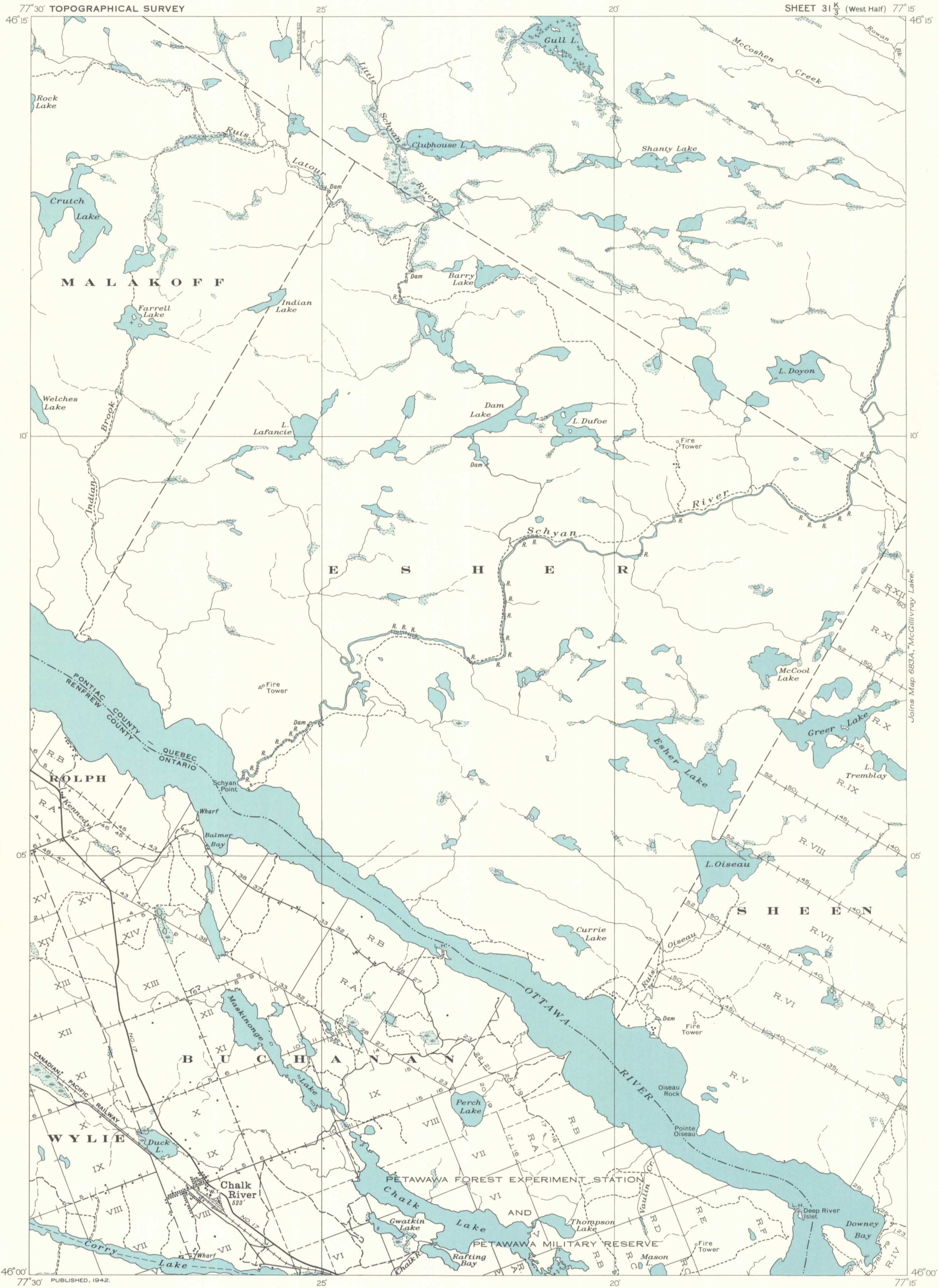
MAP 686A CHALK RIVER PONTIAC AND RENFREW COUNTIES QUEBEC AND ONTARIO Scale, 63,360 or 1 Inch to 1 Mile Approximate magnetic declination, 12° West.
