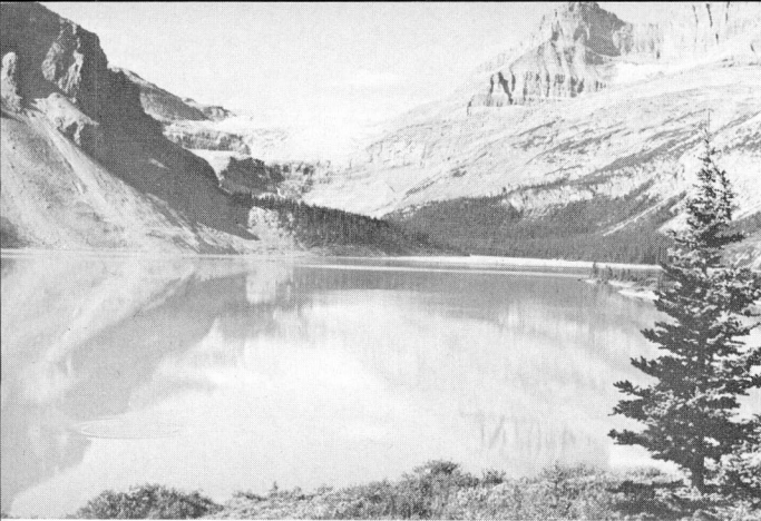
Figure 31. Bow Lake, with Bow Glacier in the distance, near the headwaters of Bow River. The mountains are made up of Lower Cambrian quartzites and shales overlain by Middle Cambrian limestones. Bow Glacier is a tongue of the Wapta ice-field, barely visible at the top of the glacier. A delta (right centre) is being built into Bow Lake by the stream of meltwater from the glacier as it carries glacial debris downwards.
