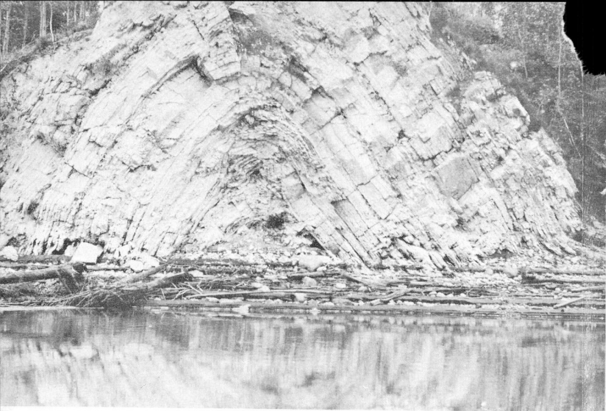
Figure 11. Rock arch or anticline.
