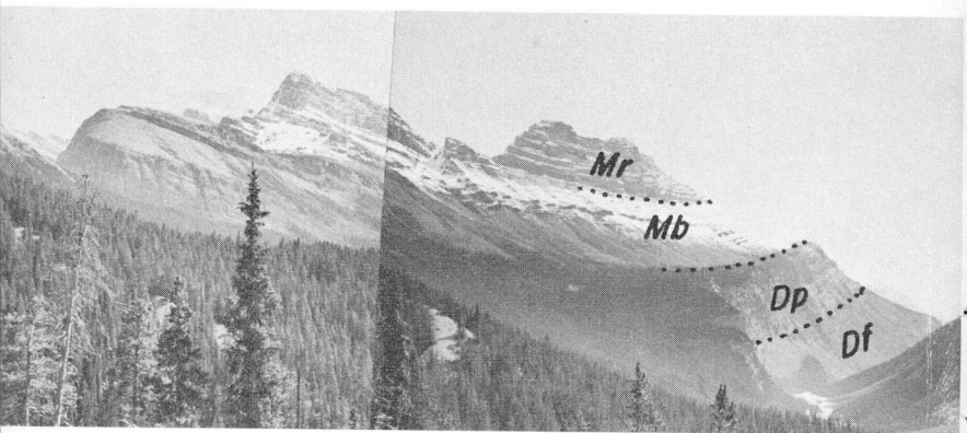
Figure 12. Cirrus Mountain, Banff-Jasper highway, as seen from near Sunwapta Pass. The rock layers bow down gently under the peak in the form of a syncline. Mr - Mississippian Rundle limestone; Mb - Banff shale; Dp - Devonian Palliser limestone; Df - Devonian Alexo and Fairholme.
