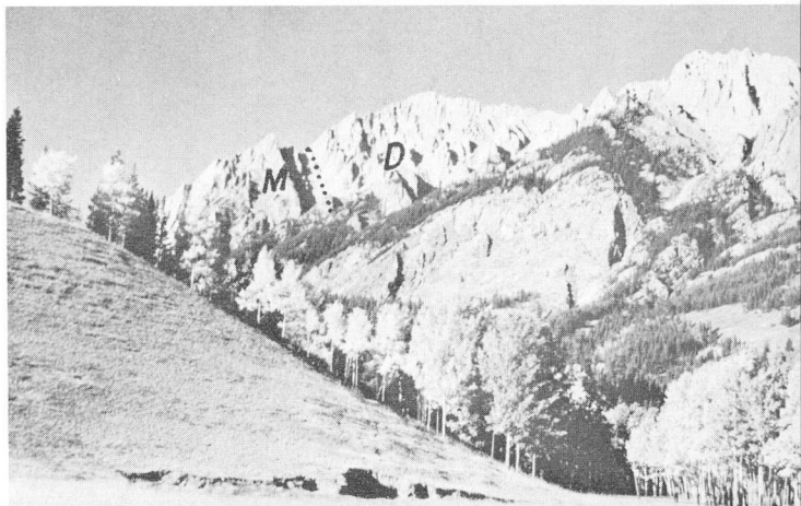
Figure 22. The Sawtooth Range. The sawtooth ridges were formed by water percolating along fractures or joints in the steeply dipping Mississippian (M) and Devonian (D) limestone strata.
