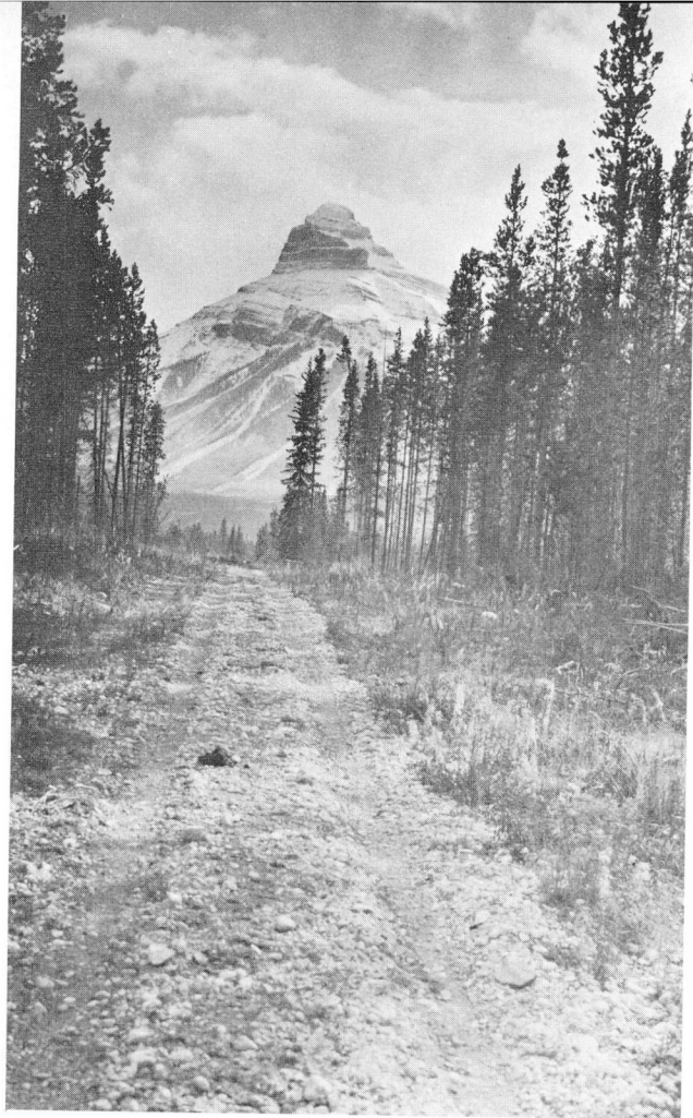
Figure 28. Pilot Mountain may be seen for a long distance up Bow River valley. It is capped by cliffs of the Mississippian Kundale formation that rest on layered Banff shales.
