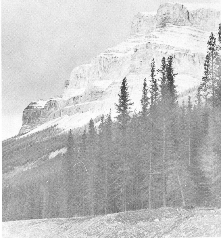
Figure 4. The stark profile of Mount Wilson exhibits the Lower Ordovician rock sequence of the Banff-Jasper highway. Tree and grass covered slopes at the base are Upper Cambrian. The cliffs are mostly massive limestone beds and the slopes are thinly layered limestones and shales. The uppermost cliff is Upper Ordovician Mount Wilson quartzite, 550 feet thick here.
