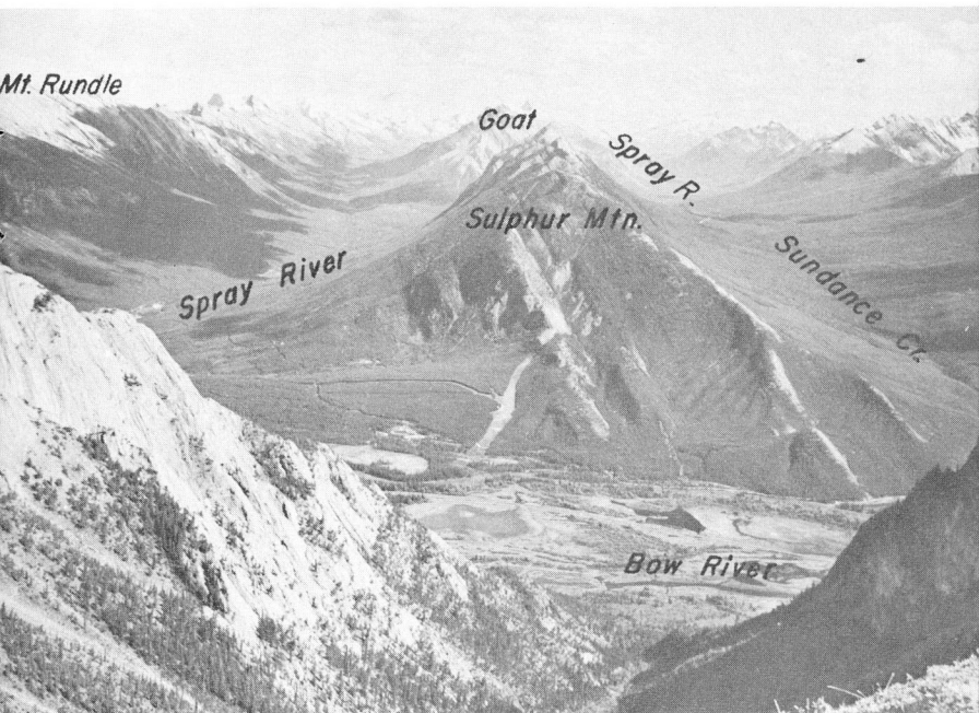
Figure 25. Sulphur Mountain, Spray and Sundance valleys from Mount Norquay with Bow River valley in the foreground. These valleys have a history of stream piracy. The Bow River, as the main stream, cut its valley most rapidly and the waters in the valley east of Sulphur Mountain (the present Spray River) flowed into it. The valley west of Sulphur Mountain (Sundance Creek, now), where once flowed a large stream, the early Spray, was choked by glacial drift. As a result the stream in the lower Spray River valley cut the gap between Sulphur and Goat ranges and captured the headwaters of the Spray, deflecting the main stream to the east of Sulphur Mountain. Hence we find little Sundance Creek occupying the broad valley west of Sulphur Mountain.
