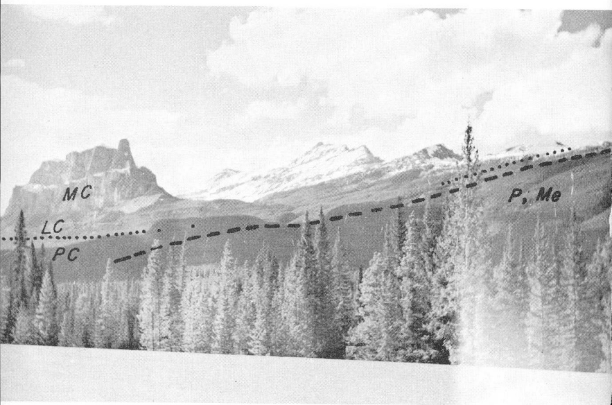
Figure 9. Mount Eisenhower as it appears today. Above the Castle Mountain thrust are Precambrian (PC) and Cambrian (LC and MC) rocks that have ridden up over late Palaeozoic (P) and Mesozoic (Me) rocks.
