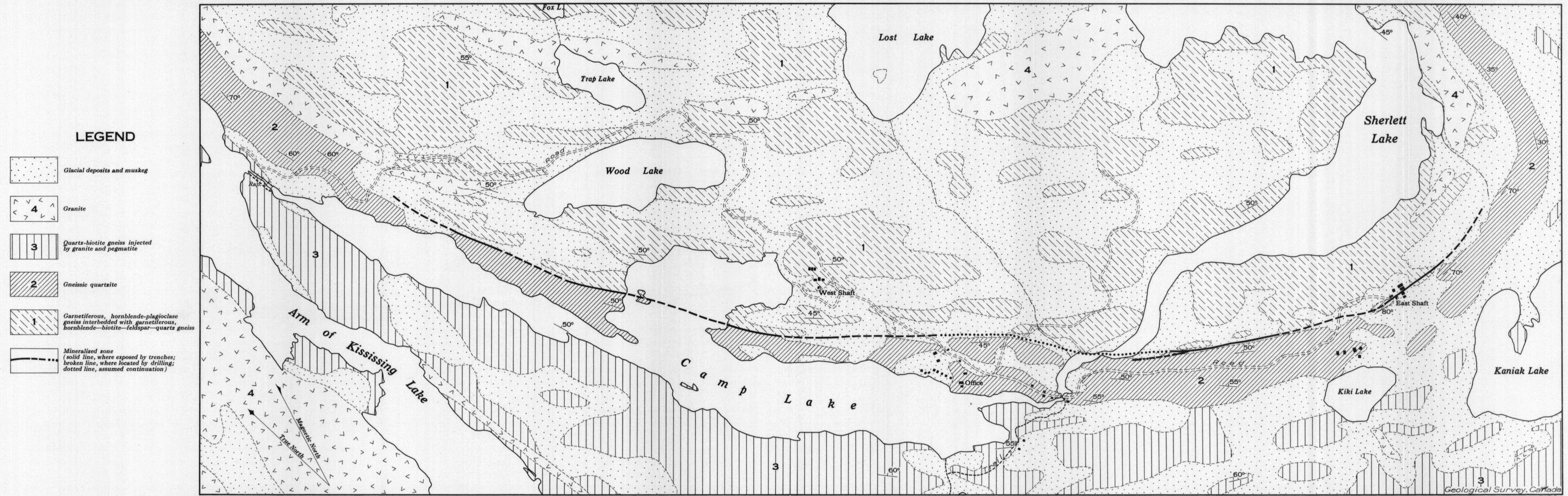
Figure 3. Sherritt-Gordon deposit, Kississing lake area, northwest Manitoba.
