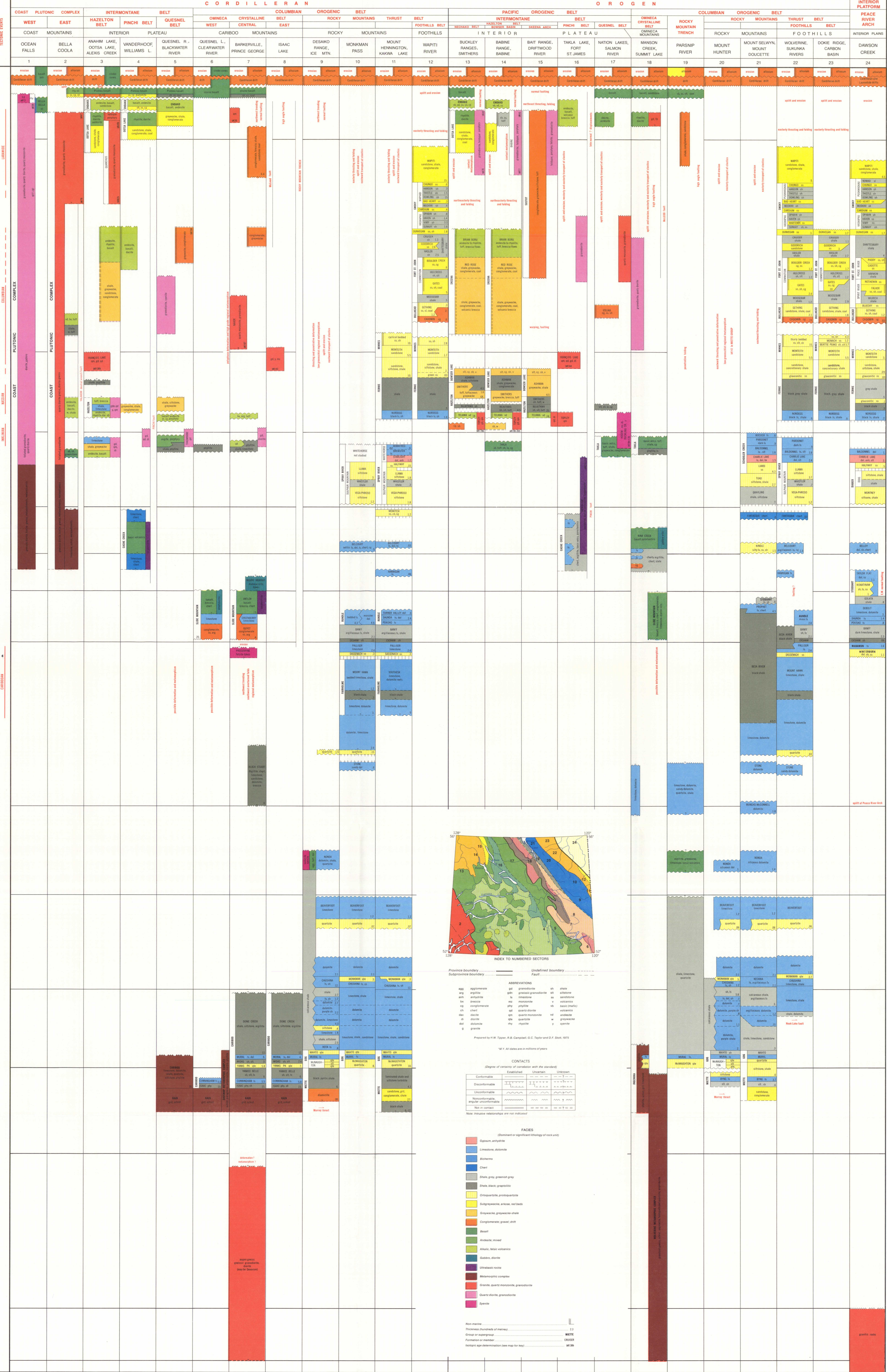
Geotectonic Correlation Chart for Sheet 93, Parsnip River, Map 1424A
