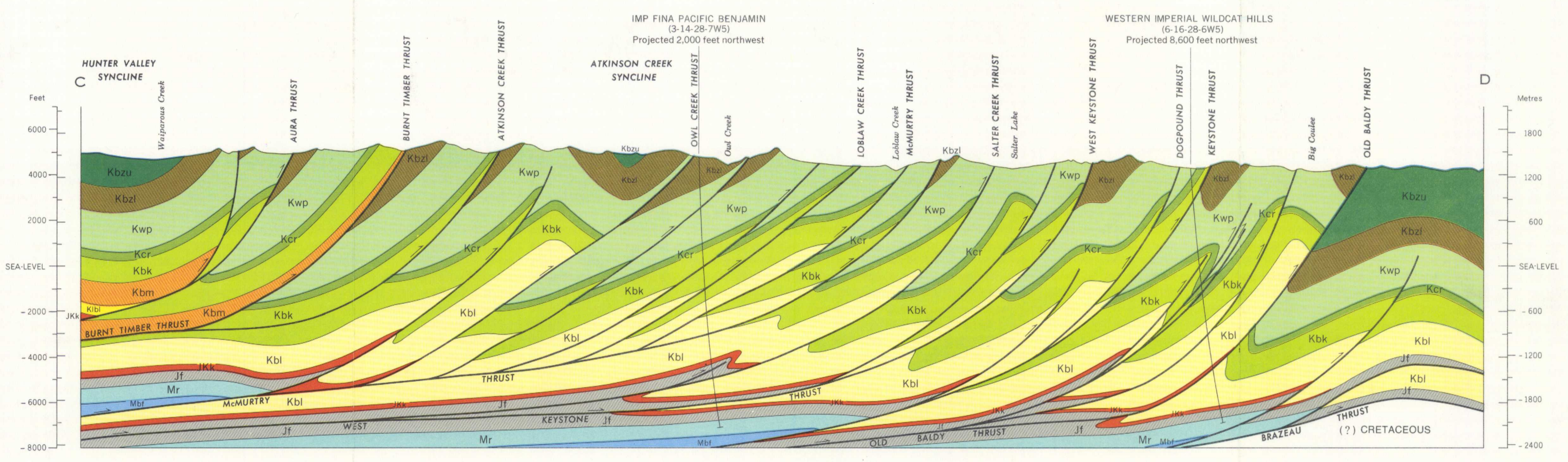
Structure cross-section C-D
