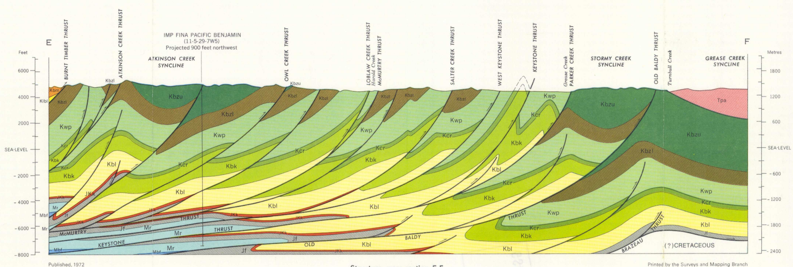
Structure cross-section E-F
