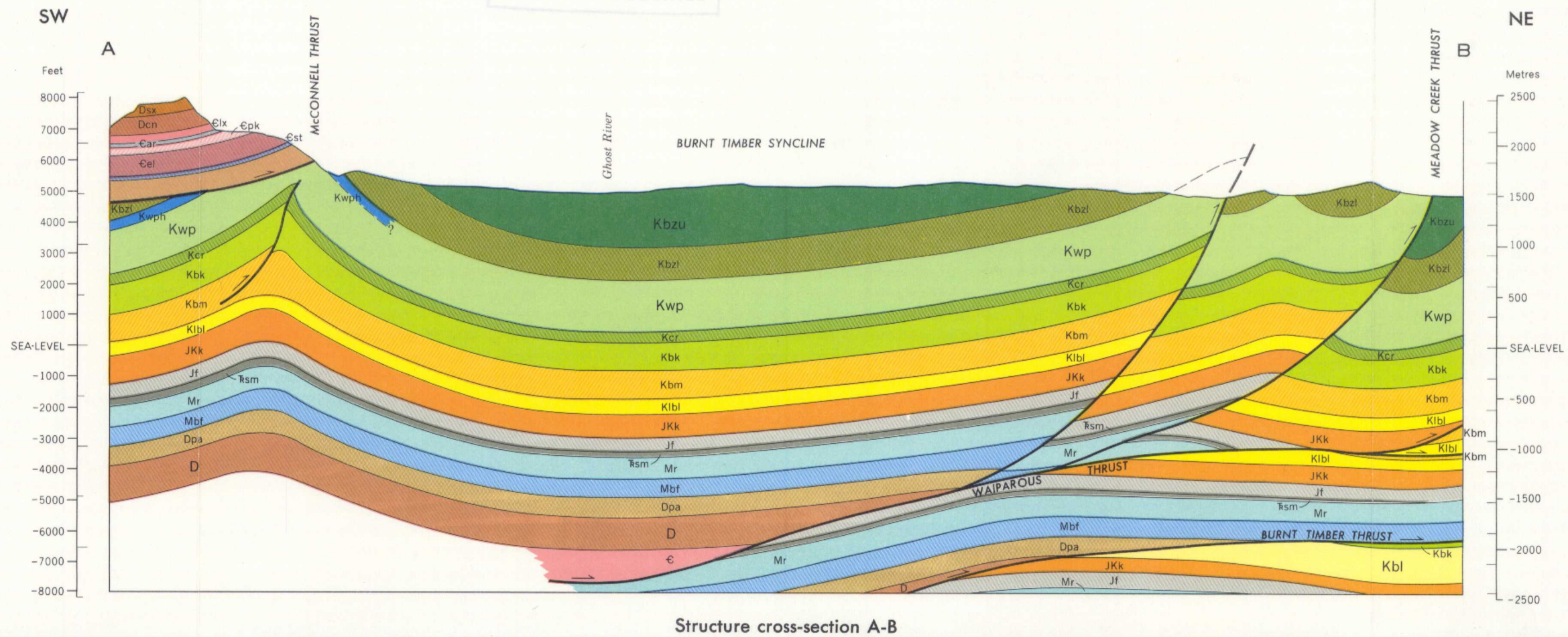
Structure cross-section A-B
