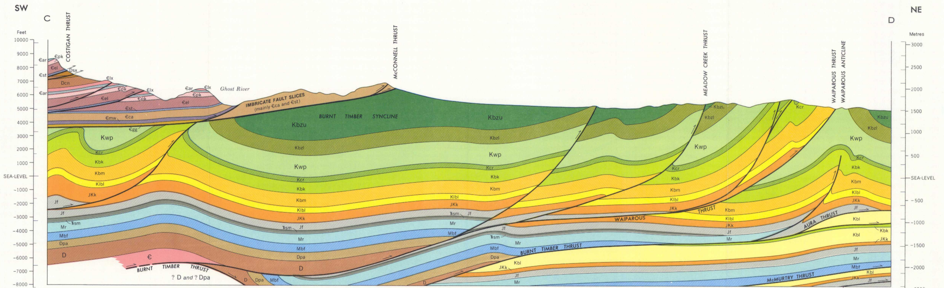
Structure cross-section C-D
