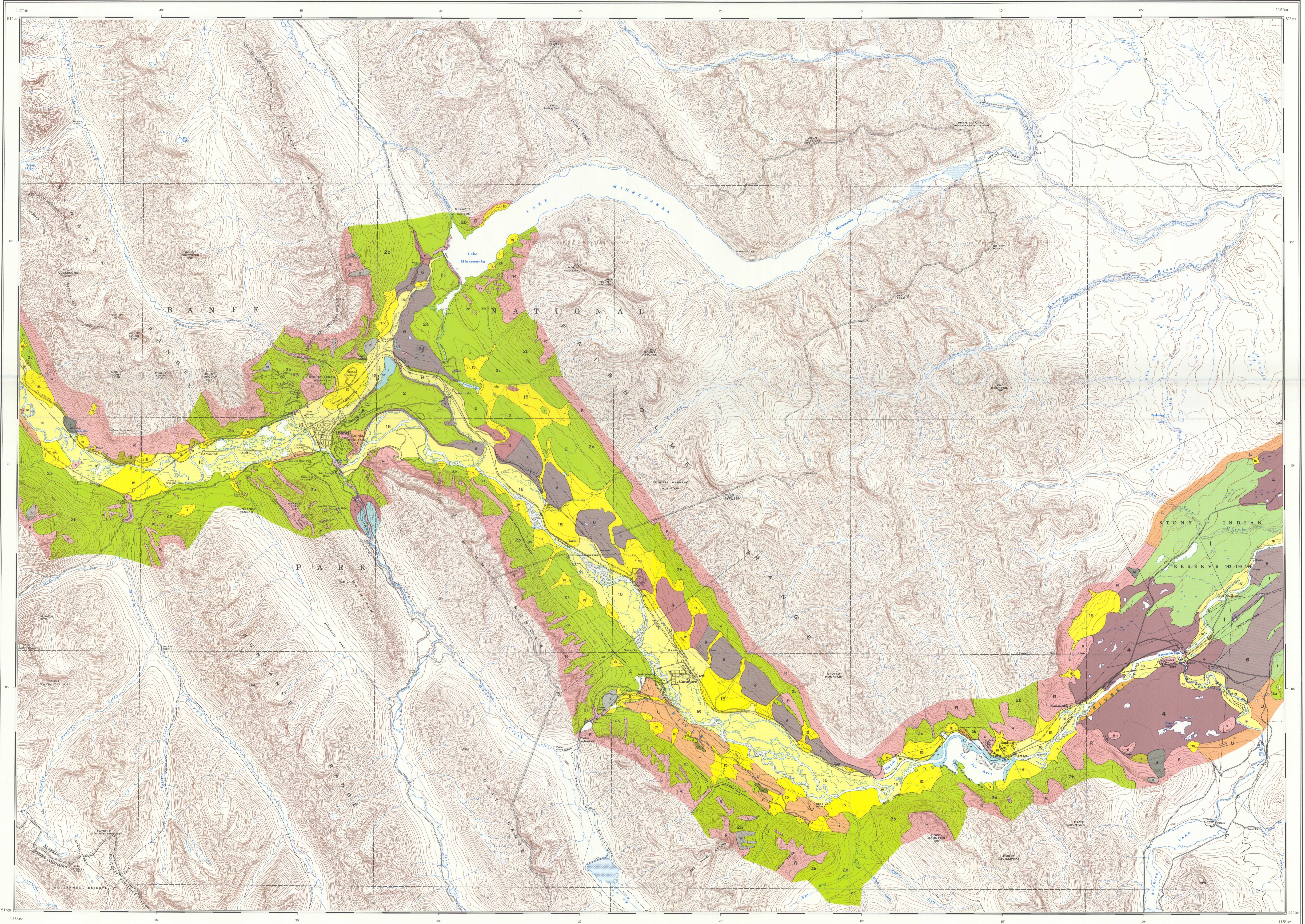
MAP 1324A SURFICIAL GEOLOGY BANFF AREA WEST OF FIFTH MERIDIAN (Sheet 2) ALBERTA Scale 1:50,000
