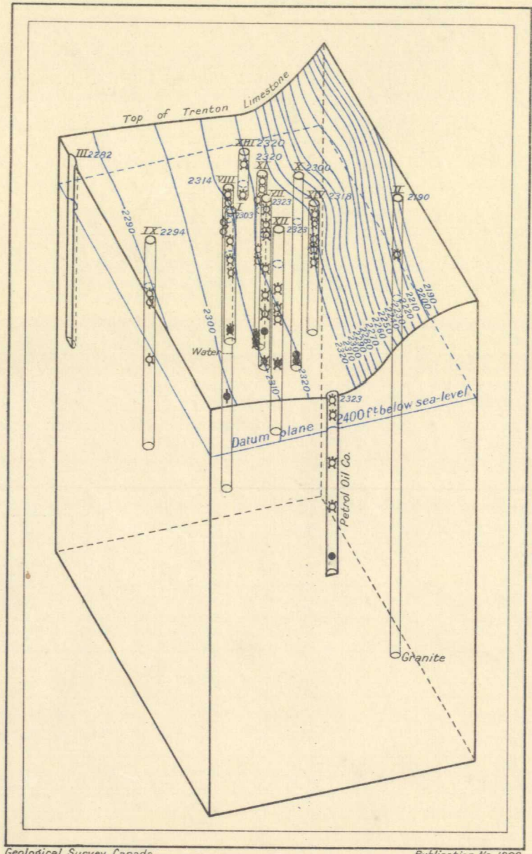
Block diagram (30° from the horizontal) illustrating the occurrence of Gas and Oil in the Trenton Limestone of Dover West Tp., Kent Co., Ontario.
