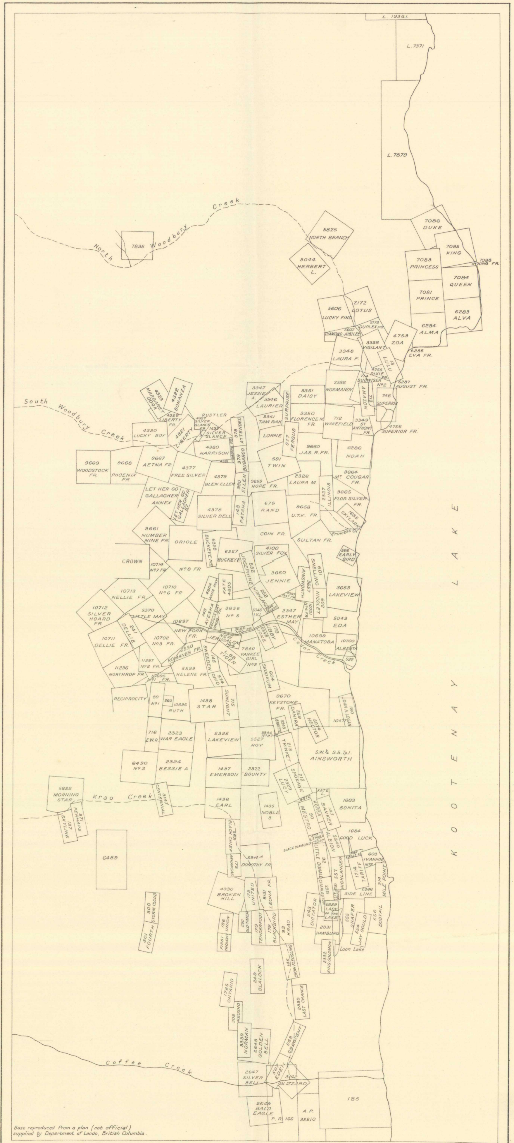
Diagram showing mineral claims, Ainsworth Mining Camp, Kootenay District, British Columbia.
