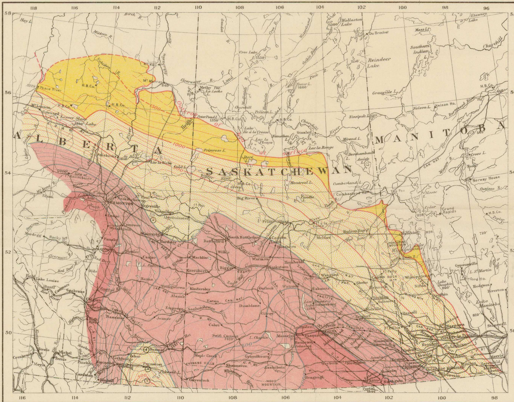
Structure contours showing Gas Horizon near base of Colorado Group.
