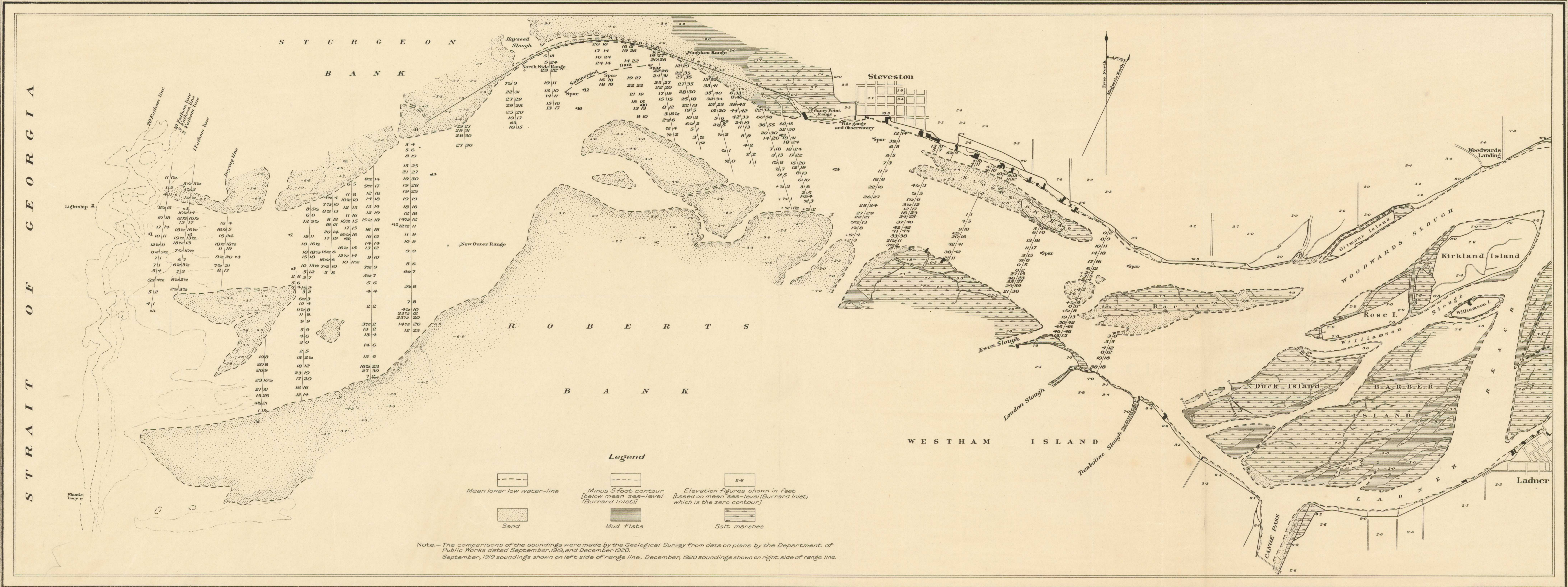
Comparative soundings, Fraser River, between Woodwards Landing and Strait of Georgia, British Columbia
