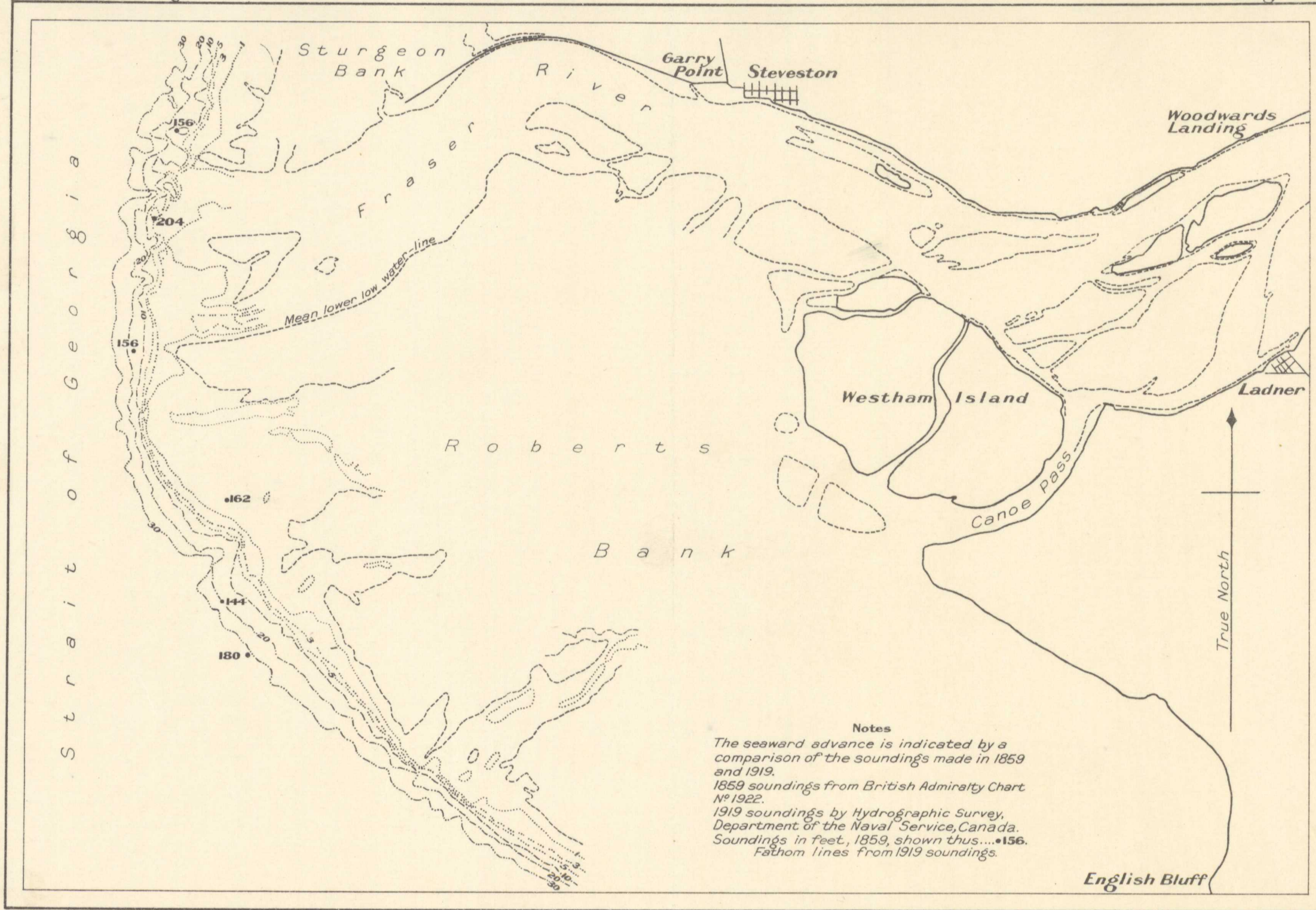
Diagram showing seaward advance of Fraser River Delta, British Columbia.
