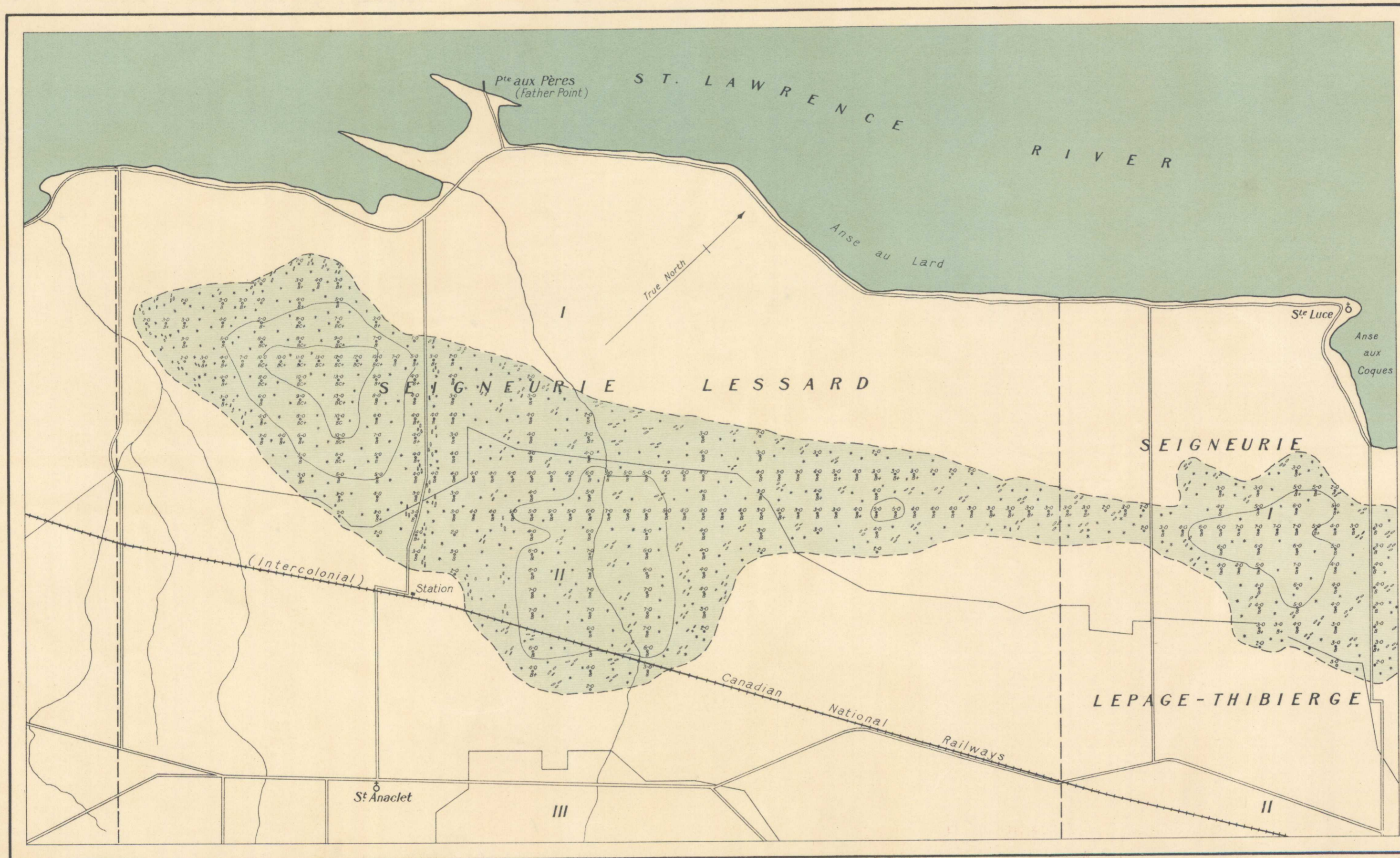
St. Anaclet Peat Bog, Lessard and Lepage-Thibierge seigniories, Rimouski county, Quebec.
