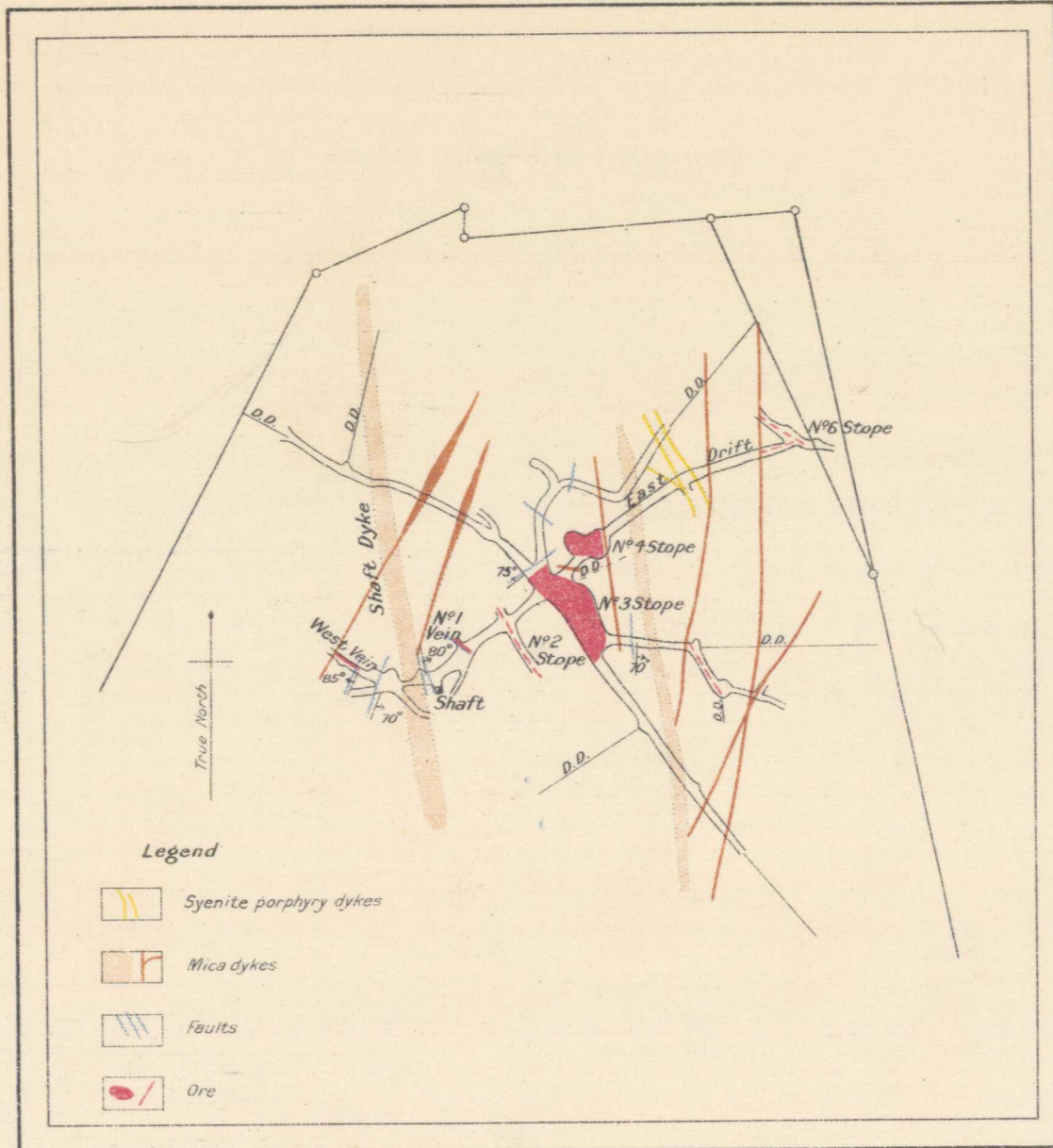
Plan of 850-foot level White Bear Mine, Rossland, B.C.
