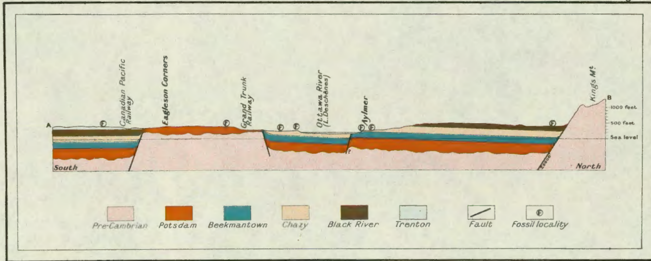
Cross-section from Kings Mountain through Aylmer, Quebec
