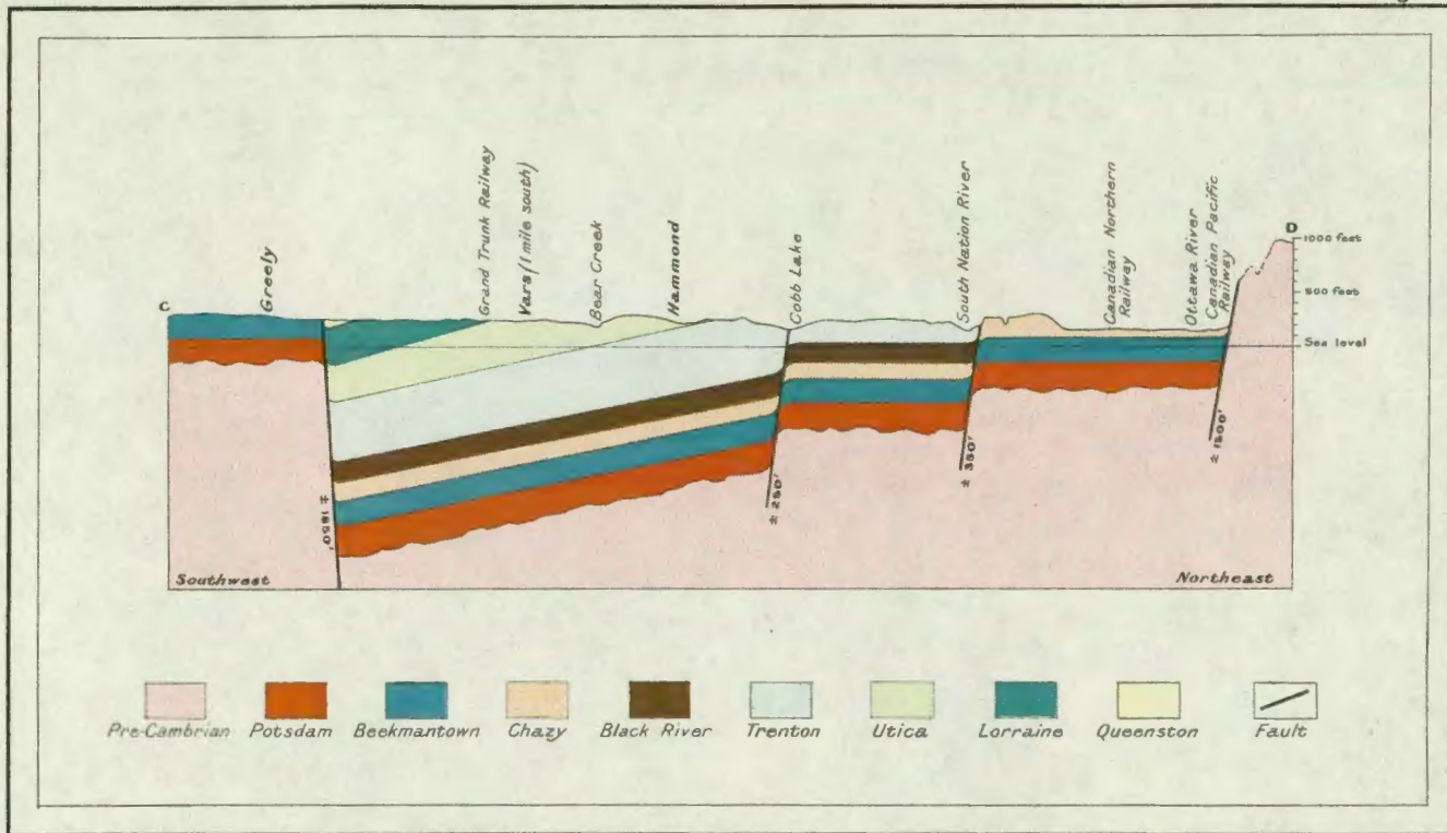
Cross-section to Vars, Ontario from the Laurentian Plateau near Montebello, Quebec
