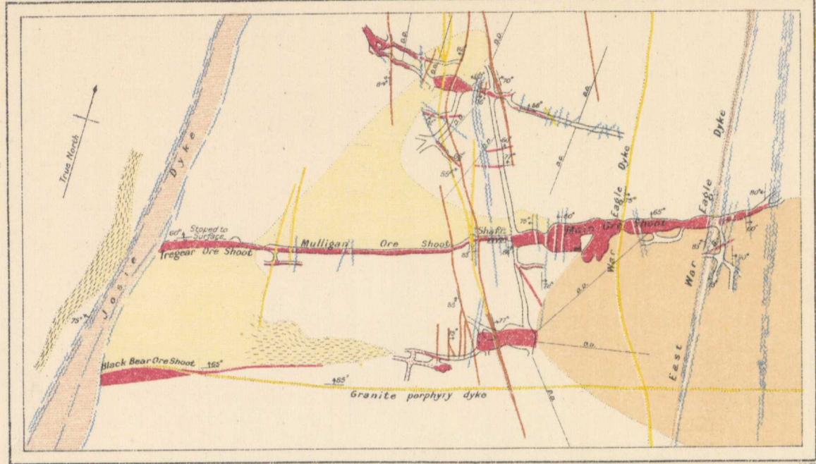
Plan of 150-foot level (elevation 3451 feet above sea-level) Le Roi Mine, Rossland, B.C.
