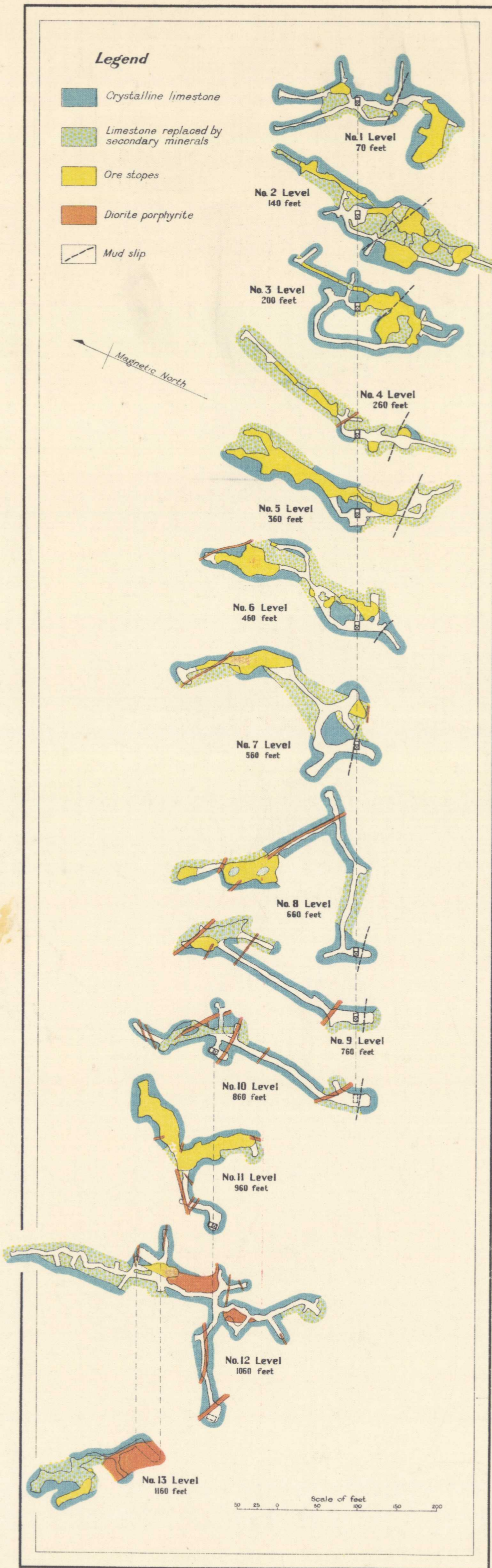
Plans of Levels, Marble Bay Mine, Texada Island, B. C. (From surveys by management)
