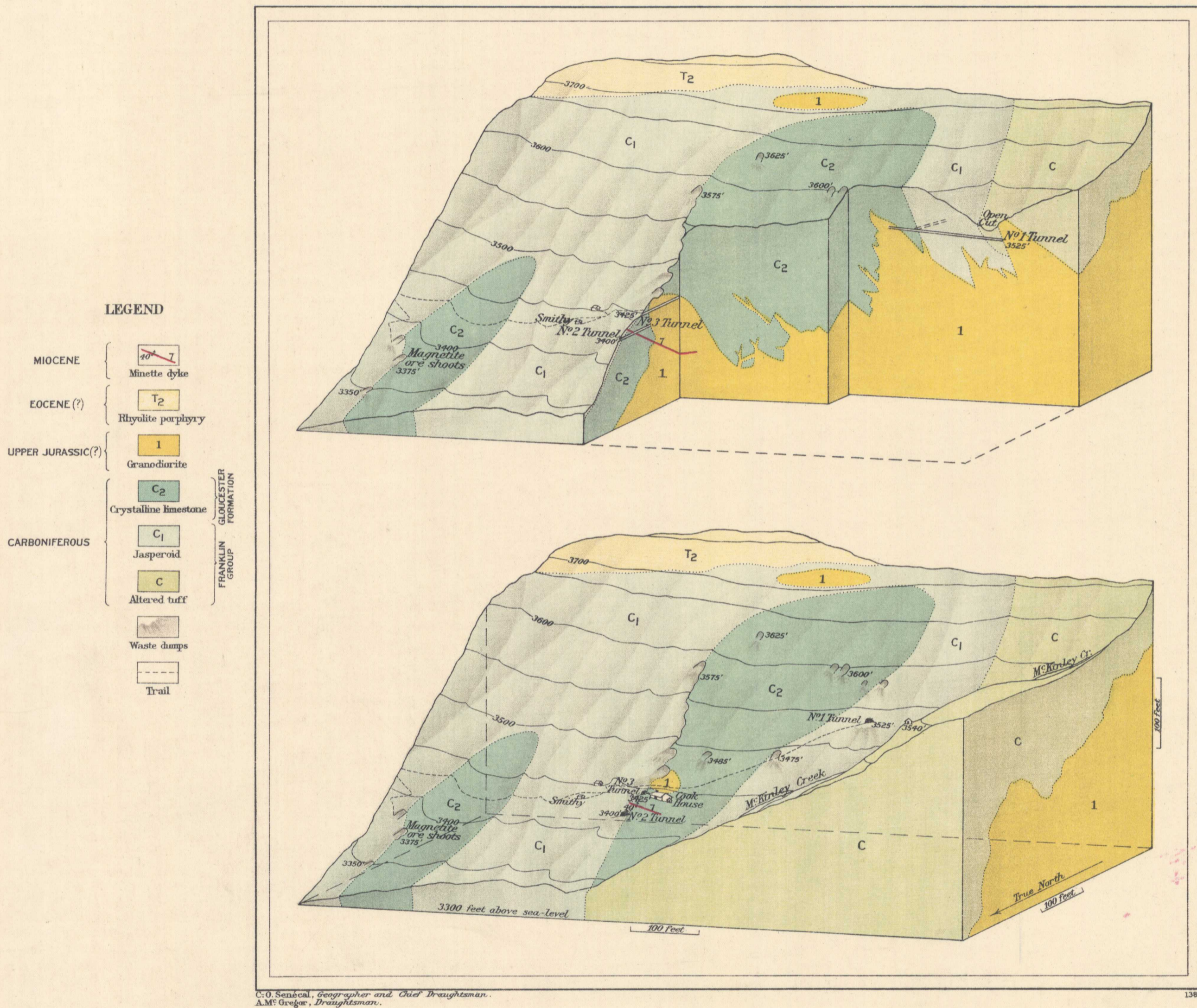
FIG. 16 - BLOCK DIAGRAM OF MCKINLEY MINE, FRANKLIN MINING CAMP, WEST KOOTENAY, B. C.
