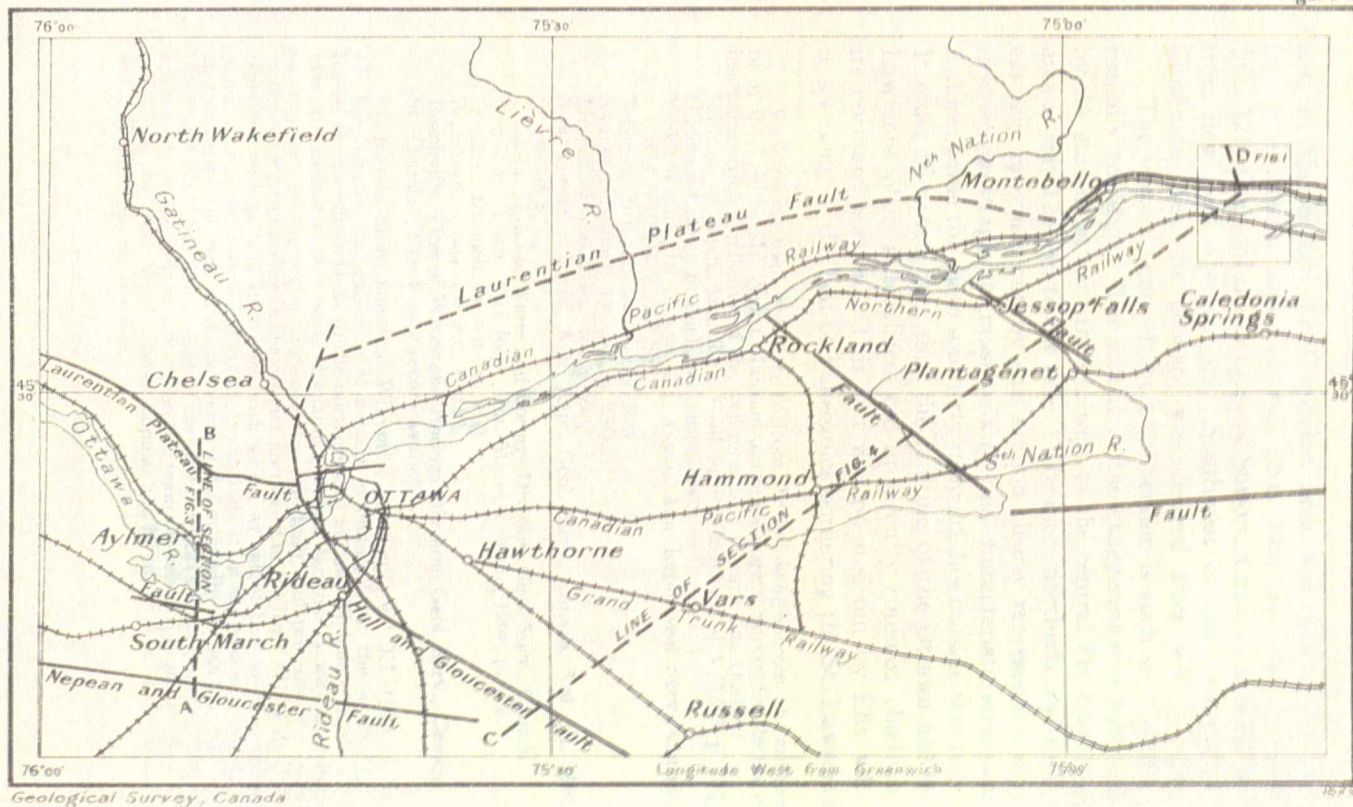
Outline map of the Ottawa District showing principal faults and lines of cross-sections
