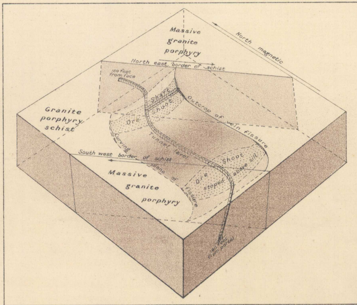
Fig. 3. Block diagram of the Tamarac fissure vein showing structural relations of the ore shoots. The vein dips at an angle of 35 degrees and is curved as indicated.
