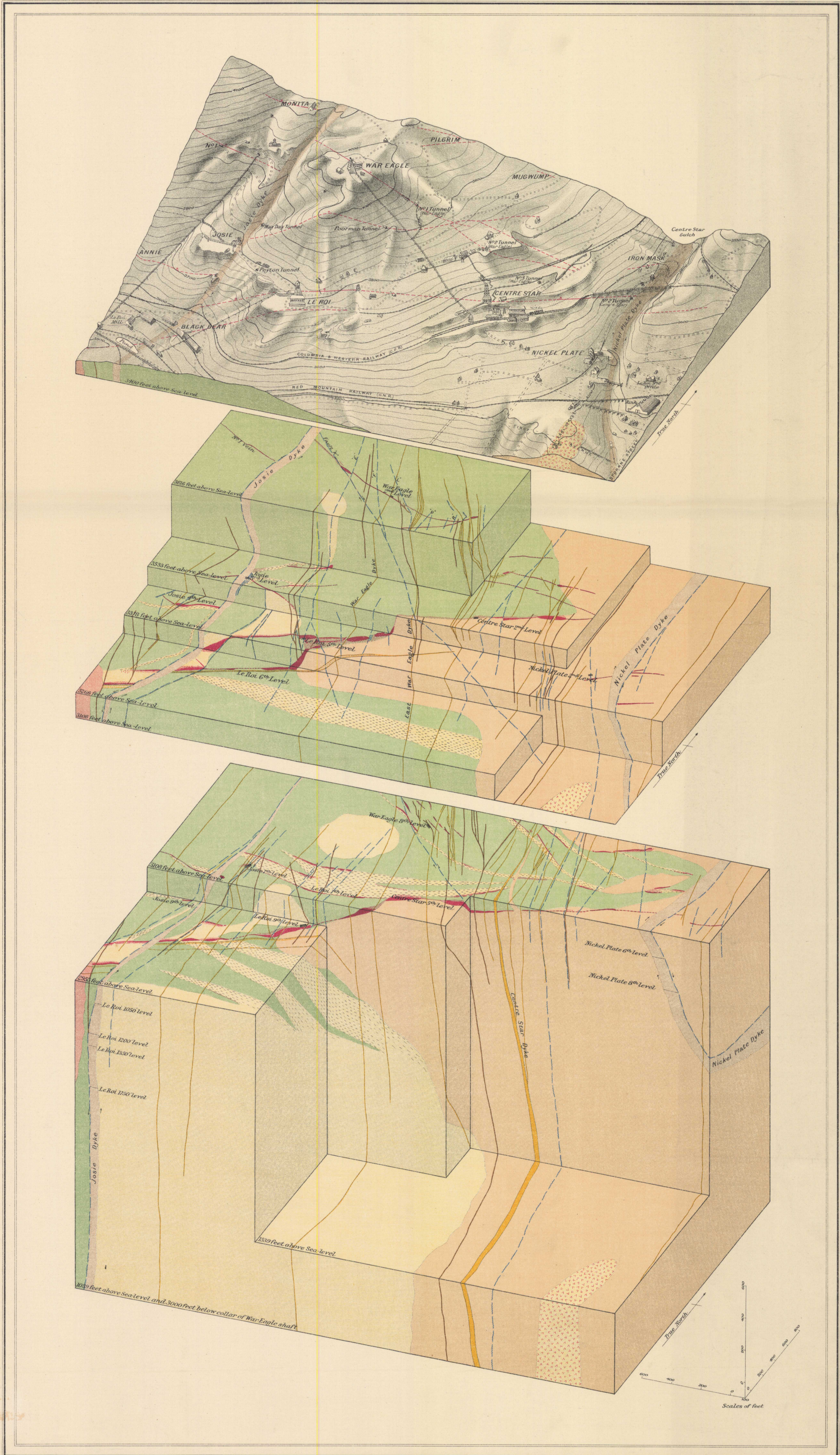
STEREOGRAMS OF A BLOCK OF ORE-BEARING COUNTRY, ROSSLAND, B.C.
