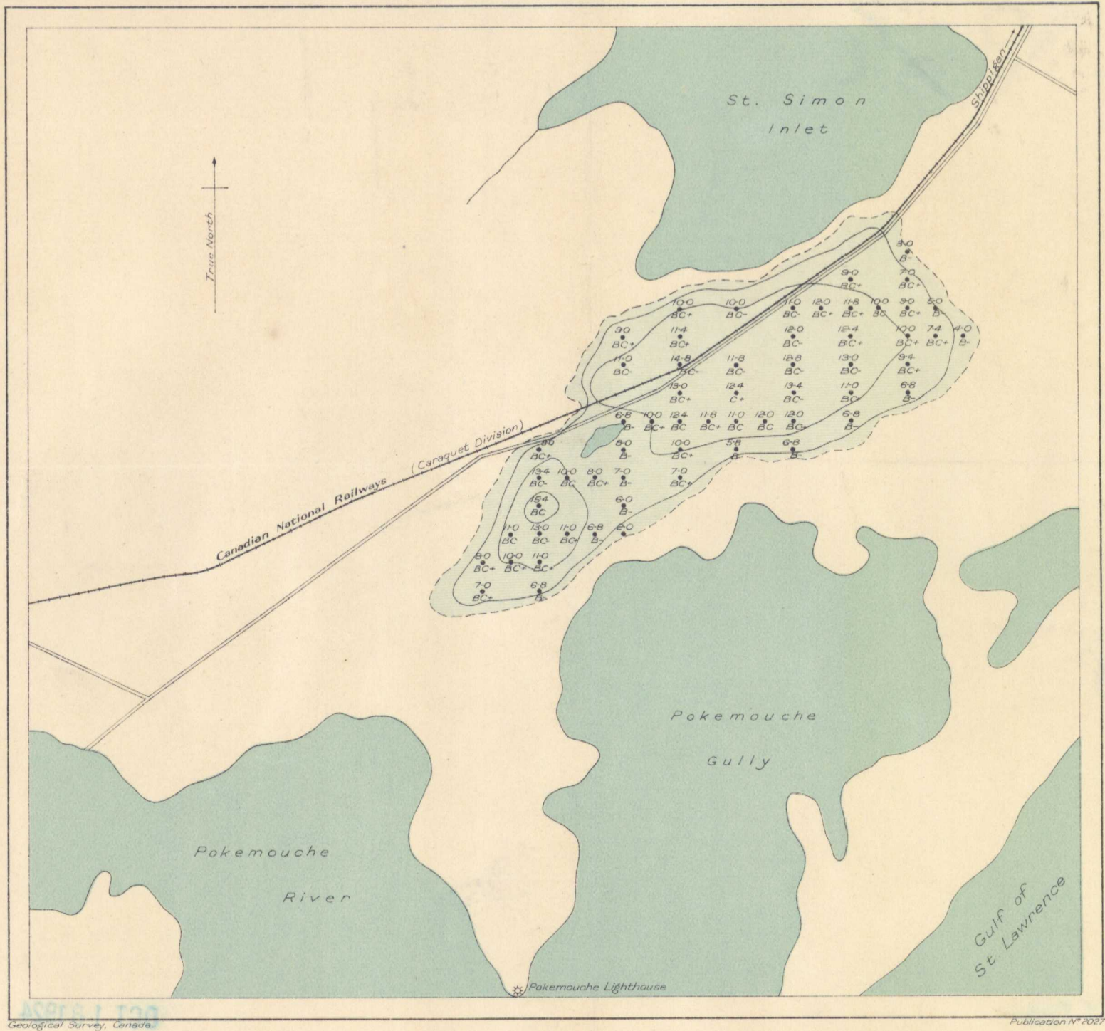
Pokemouche Peat Litter Bog, Gloucester County, New Brunswick.
