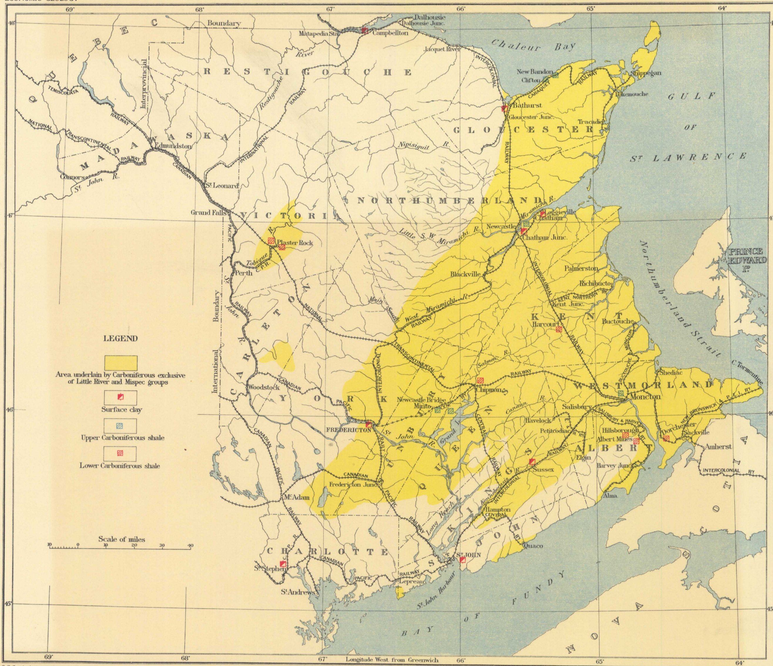
NEW BRUNSWICK - CARBONIFEROUS AREAS, AND POSITIONS OF CERTAIN SHALE AND CLAY DEPOSITS.
