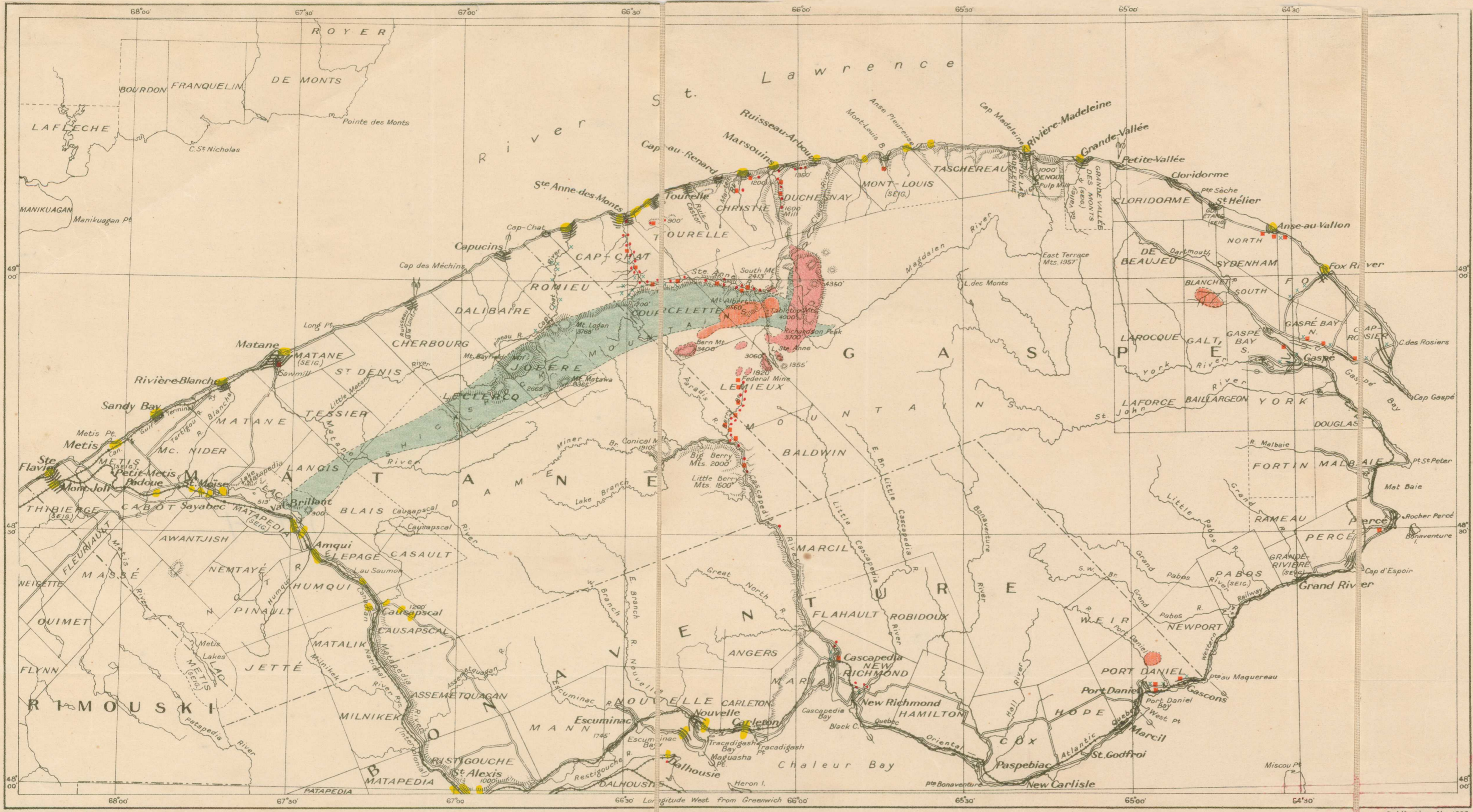
Diagram showing direction of movement of local glaciers, Gaspé Peninsula, Quebec.
