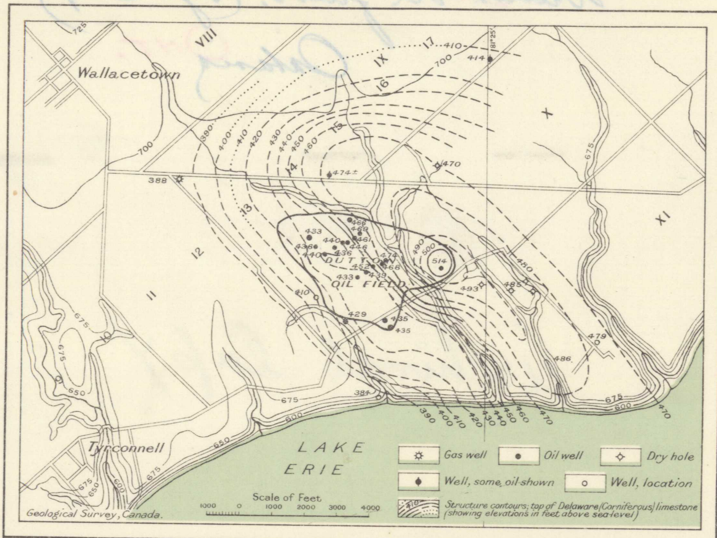
Dutton Oil field, Elgin County, Ontario.
