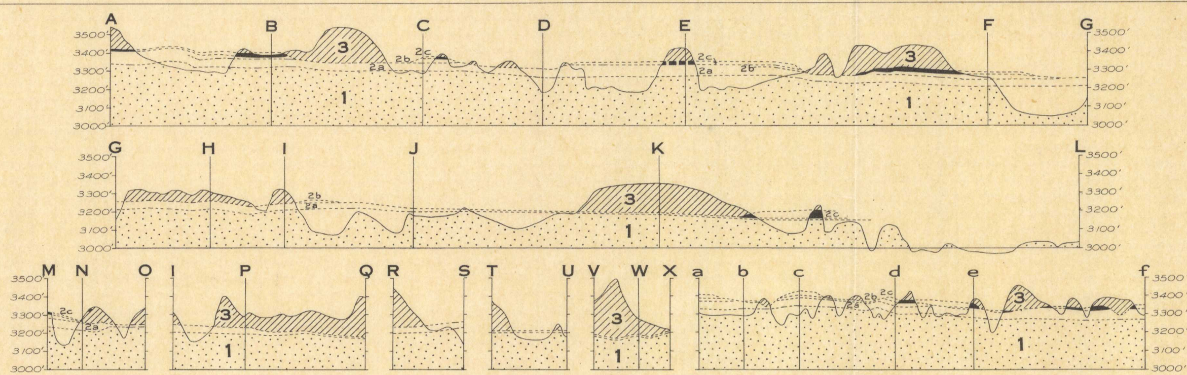
Structure sections. Vertical exaggeration, 10 times.
