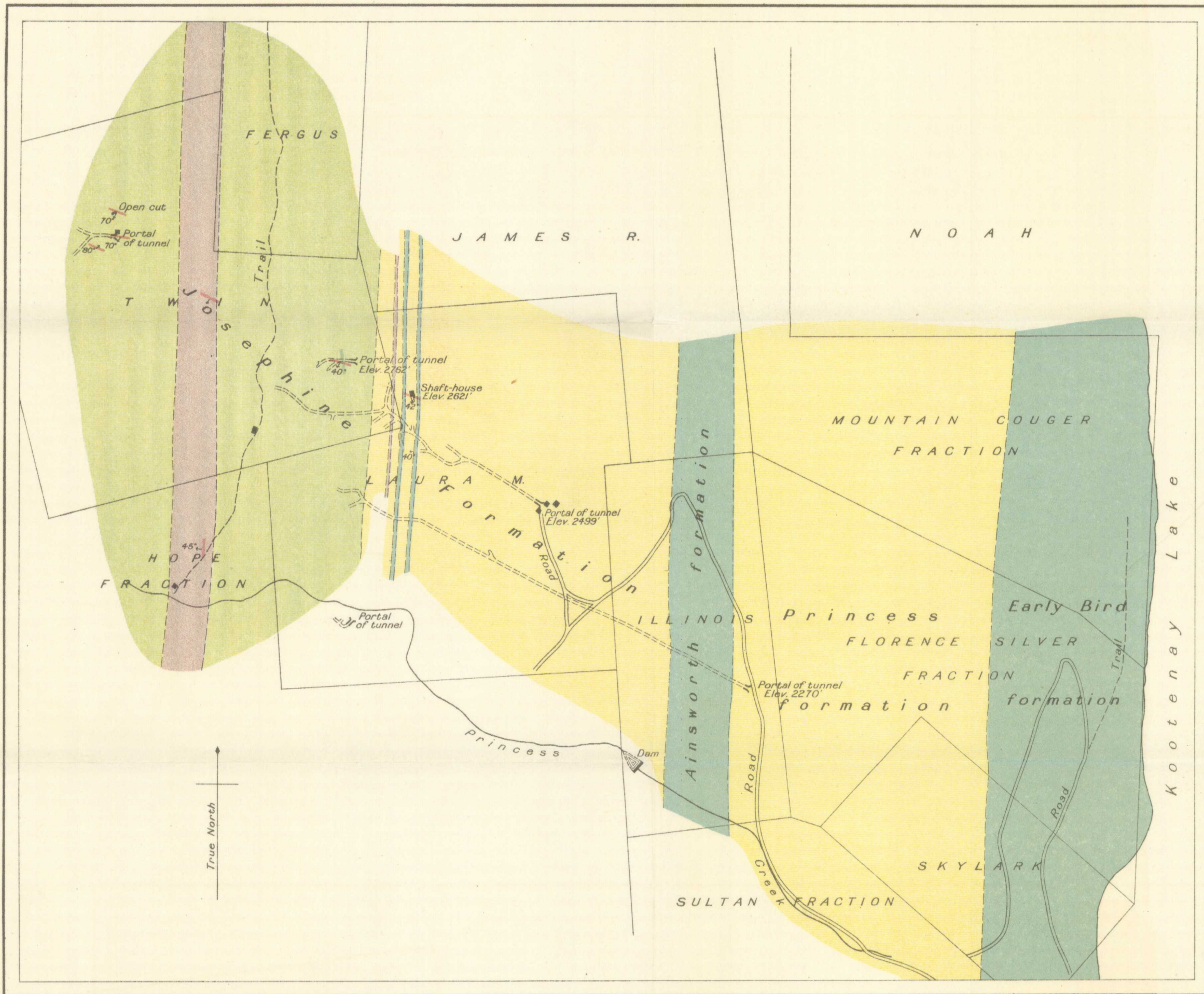
Diagram showing geology of certain mineral claims of the Florence Silver Mining Company, Ainsworth Mining Camp, Kootenay District, British Columbia.
