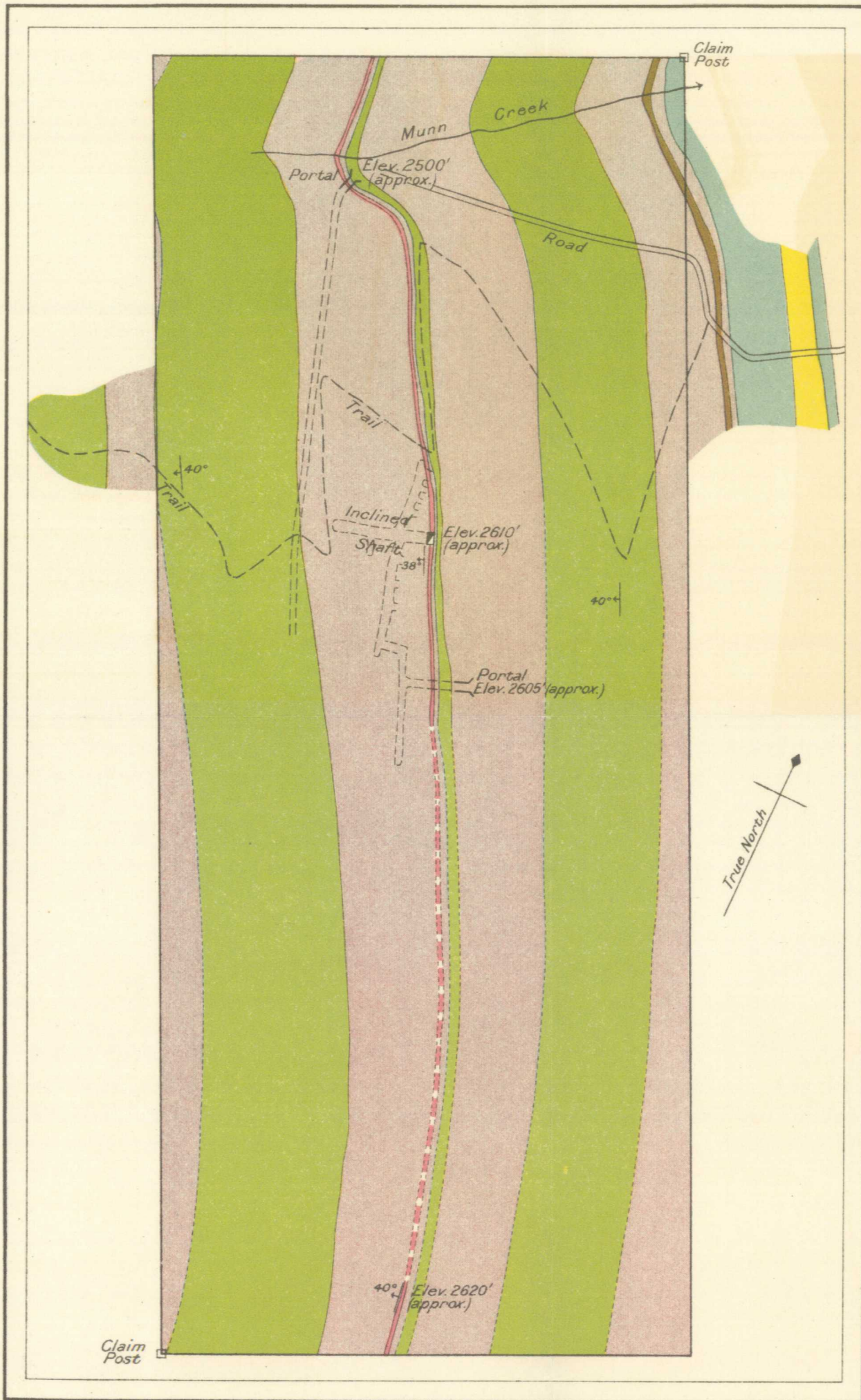
Diagram showing geology of the Spokane mineral claim, Ainsworth Mining Camp, Kootenay District, British Columbia.
