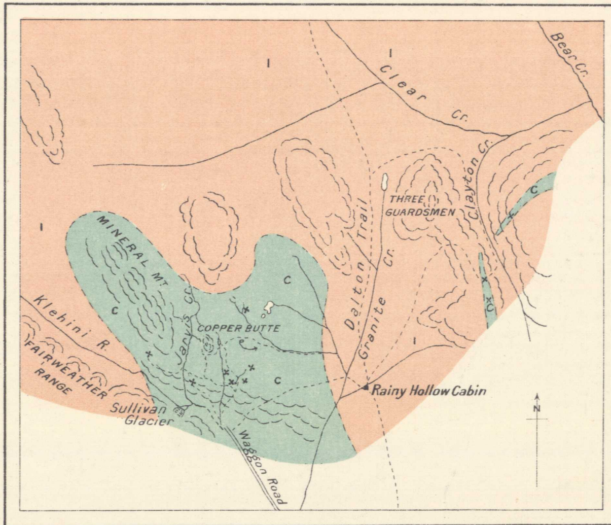
Diagram showing the geology of Rainy Hollow, Atlin Mining District B.C.
