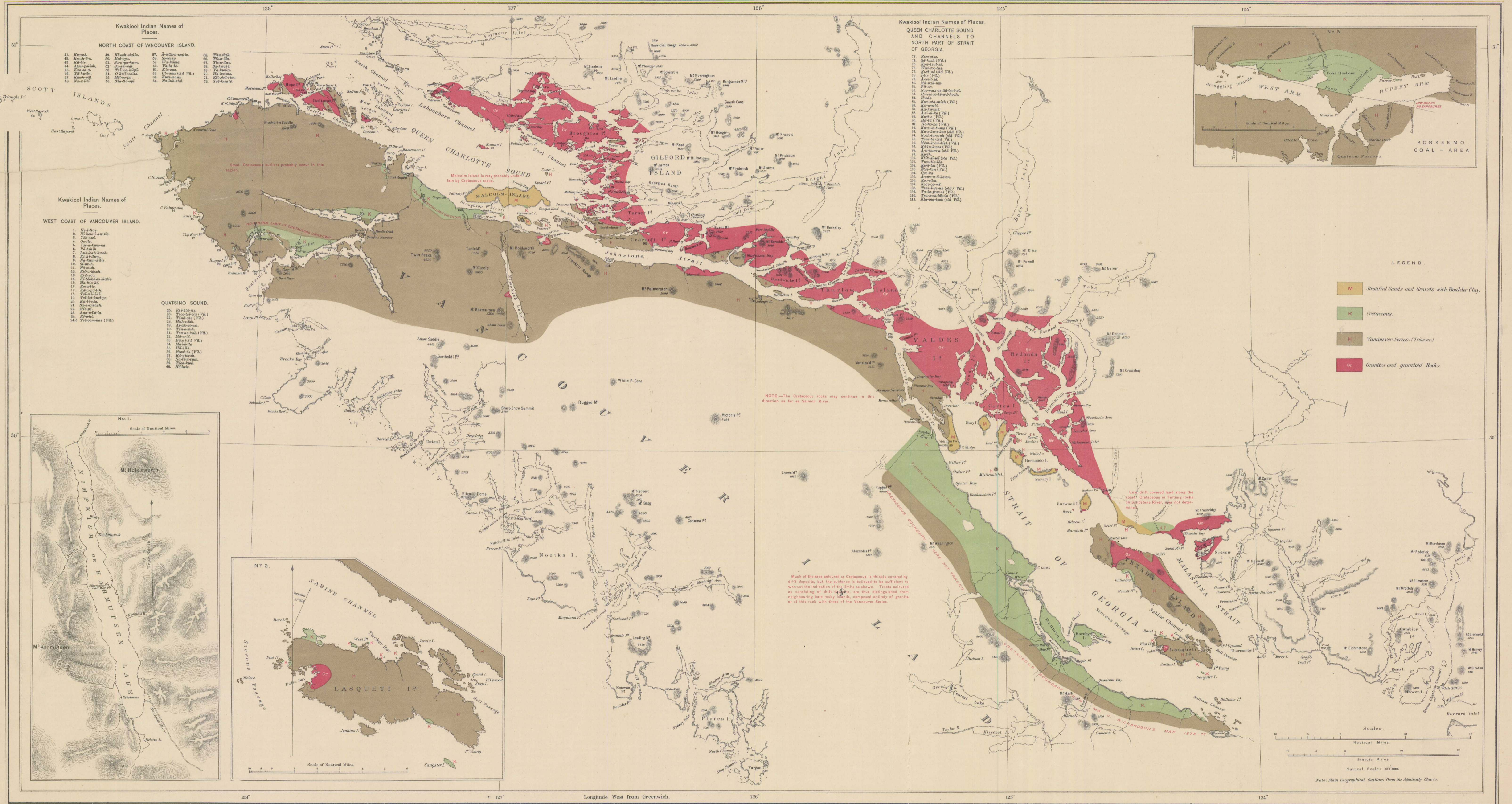
GEOLOGICAL MAP OF THE NORTHERN PART OF VANCOUVER ISLAND AND ADJACENT COASTS.
