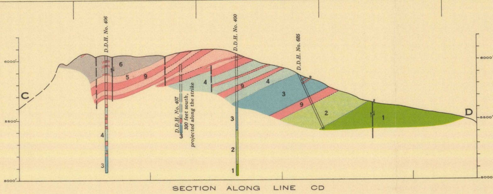
SECTION ALONG LINE CD
