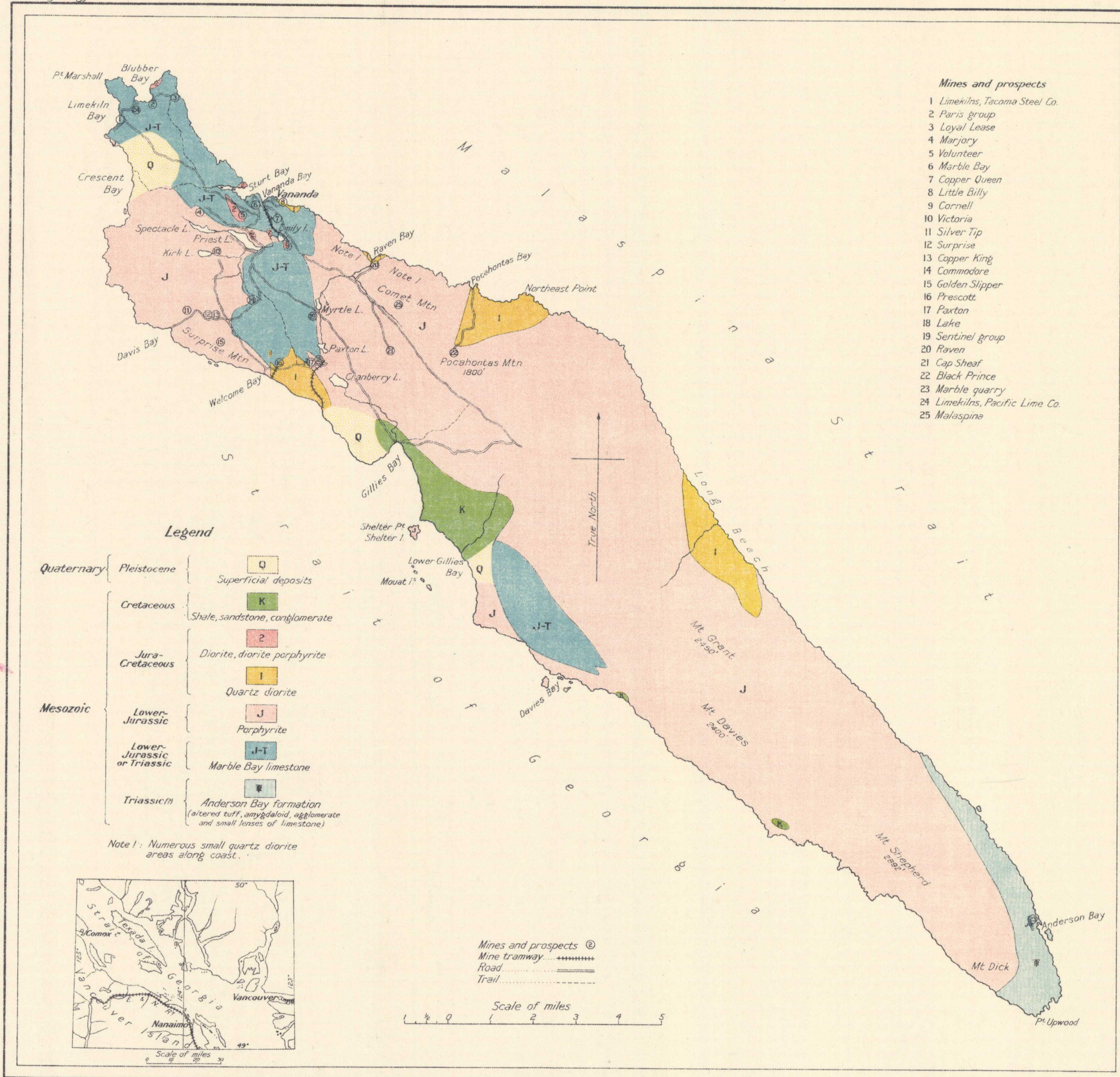
Diagram showing the geology of Texada Island, British Columbia.
