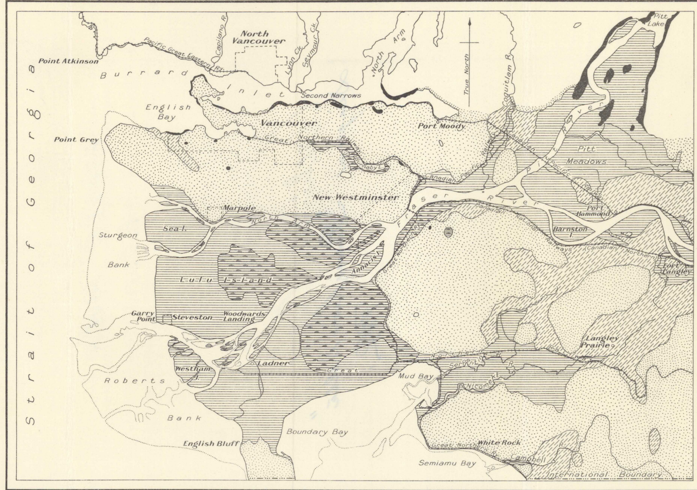
Diagram showing the distribution of surface deposits, Fraser River Delta, British Columbia.
