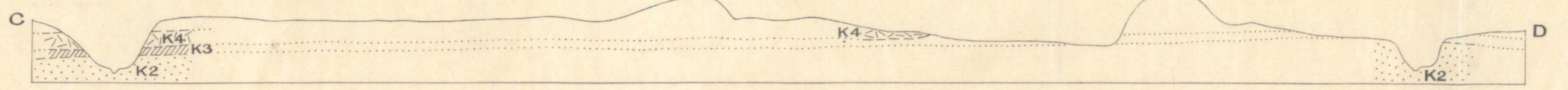
Structural section along line CD Horizontal scale, 1 inch to 6000 Feet. Vertical scale, 1 inch to 600 Feet.
