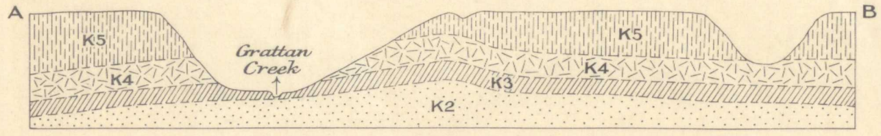
Structural section along line AB Horizontal scale, 1 inch to 2000 Feet. Vertical scale, 1 inch to 400 Feet.
