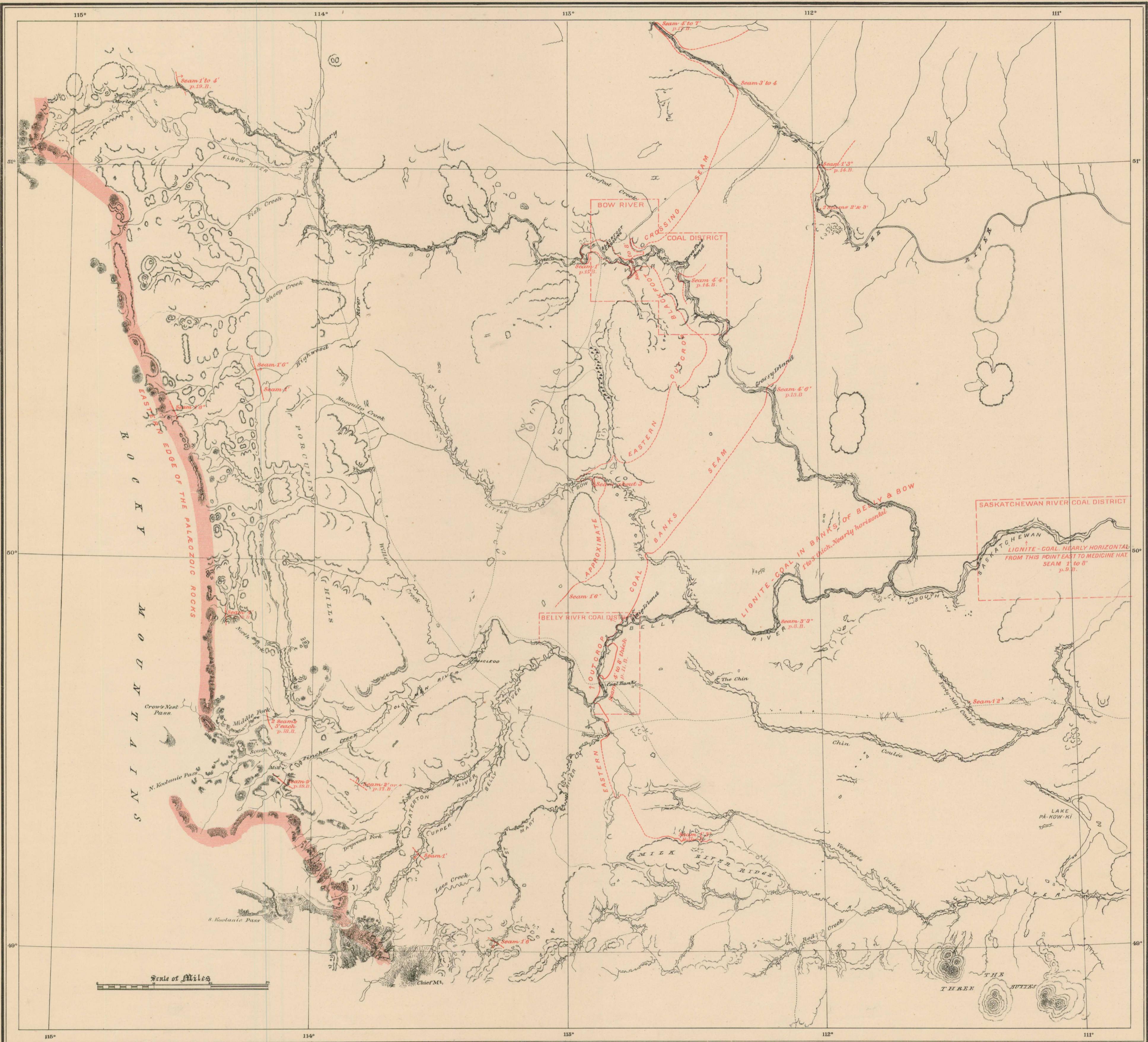
Index Map of Coal and Lignite Outcrops, Bow and Belly River District.
