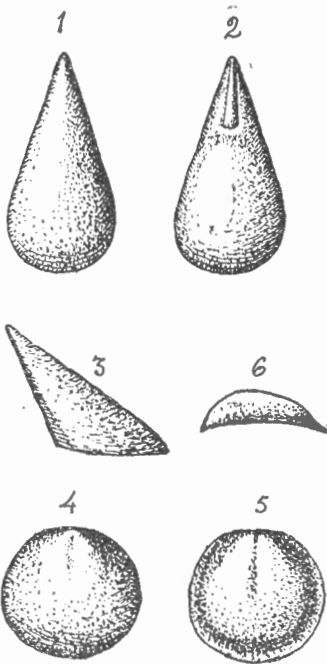
Acrothyra proavia , mut. prima — 1, Ventral valve—2, Mould of the same— 3, Same in profile—4, Dorsal valve—5, Mould of the same—6, Same in profile. All magnified \times 10 Upper Etchemin Shale, C. Breton, N. S.
