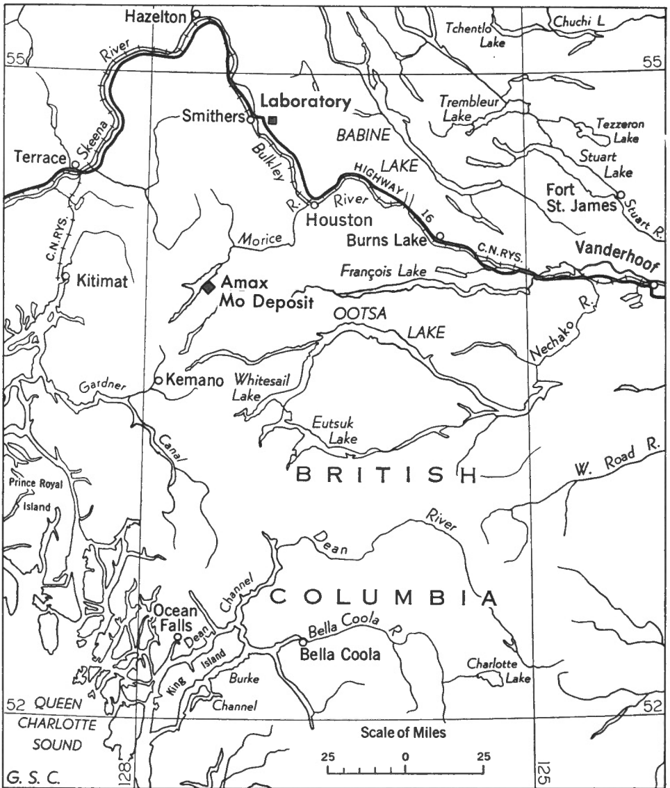
Figure 1. Index map of west-central British Columbia showing the Amax molybdenum deposit and the Trailer Laboratory site near Smithers.
