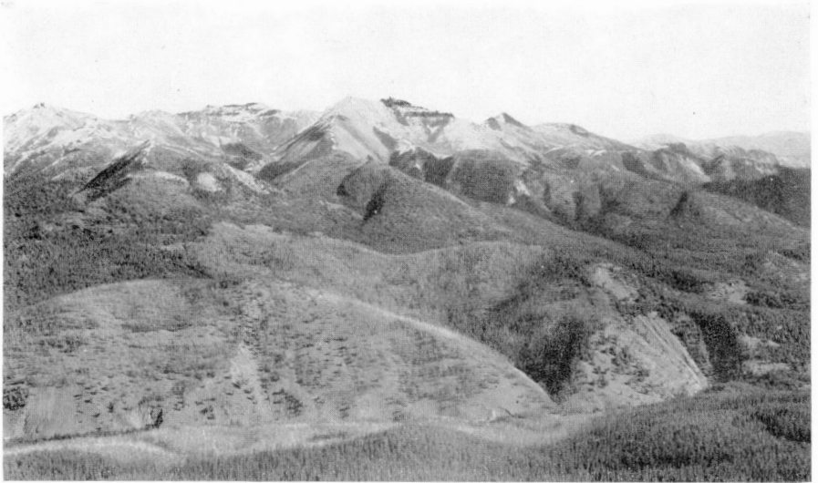
A. View northerly from near summit of Sheba Mountain across Tyaughton Creek Valley to slopes underlain by Mesozoic sedimentary formations capped by flat-lying Tertiary lavas.
