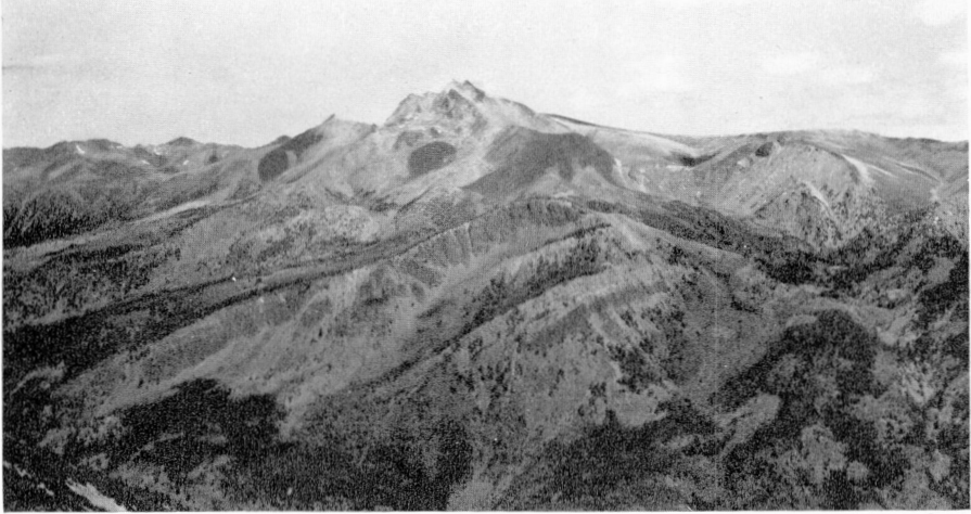
A. View northerly from Leckie Creek-Gun Creek divide across an area of mainly late Mesozoic volcanic and sedimentary rocks to Sheba Mountain, which has an elevation of 8,743 feet.
