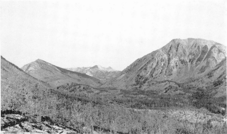
B. View northwesterly up the valley of Gun Creek from about 2 miles below the mouth of Eldorado Creek. The hills on either side are underlain mainly by Mesozoic sedimentary formations.
