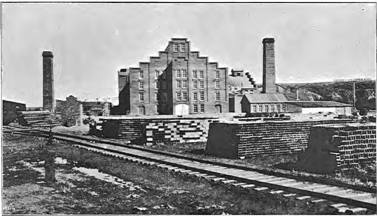
Works of the Alberta Clay Product Company, Medicine Hat, Alta.
