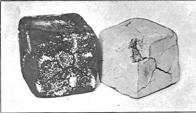
Cubes of clay, showing the cracking which occurred in air drying. Preheating prevented this.
