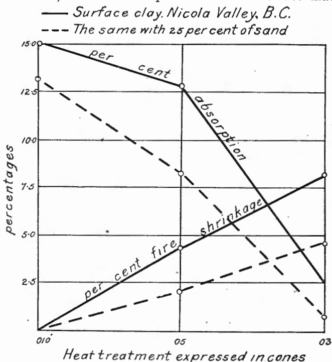
FIG. 6.—Absorption and fire shrinkage curves of surface clay from Nicola valley, B.C.
