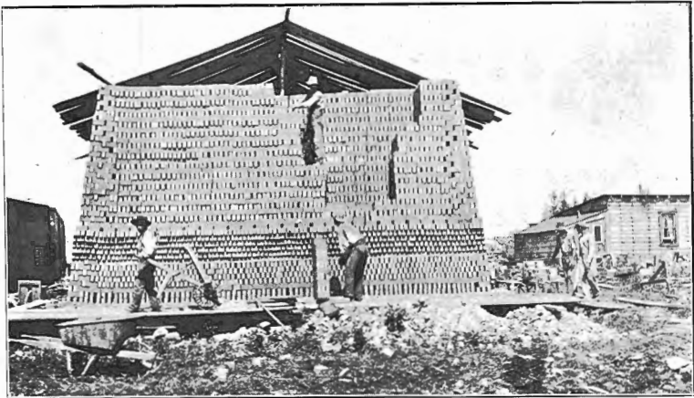
Setting green bricks in scove kiln, Acme brick works, Edmonton, Alta.
