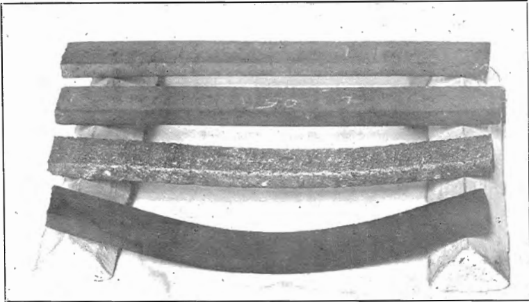
Showing the method used for setting bars of clay in kiln for warpage test.
