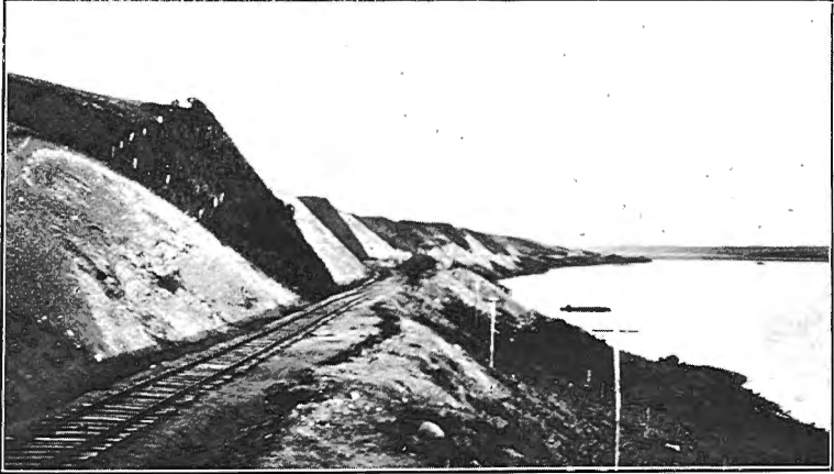
Railway cuttings in Niobrara shale and boulder clay. West shore of Lost Mountain lake, Sask.
