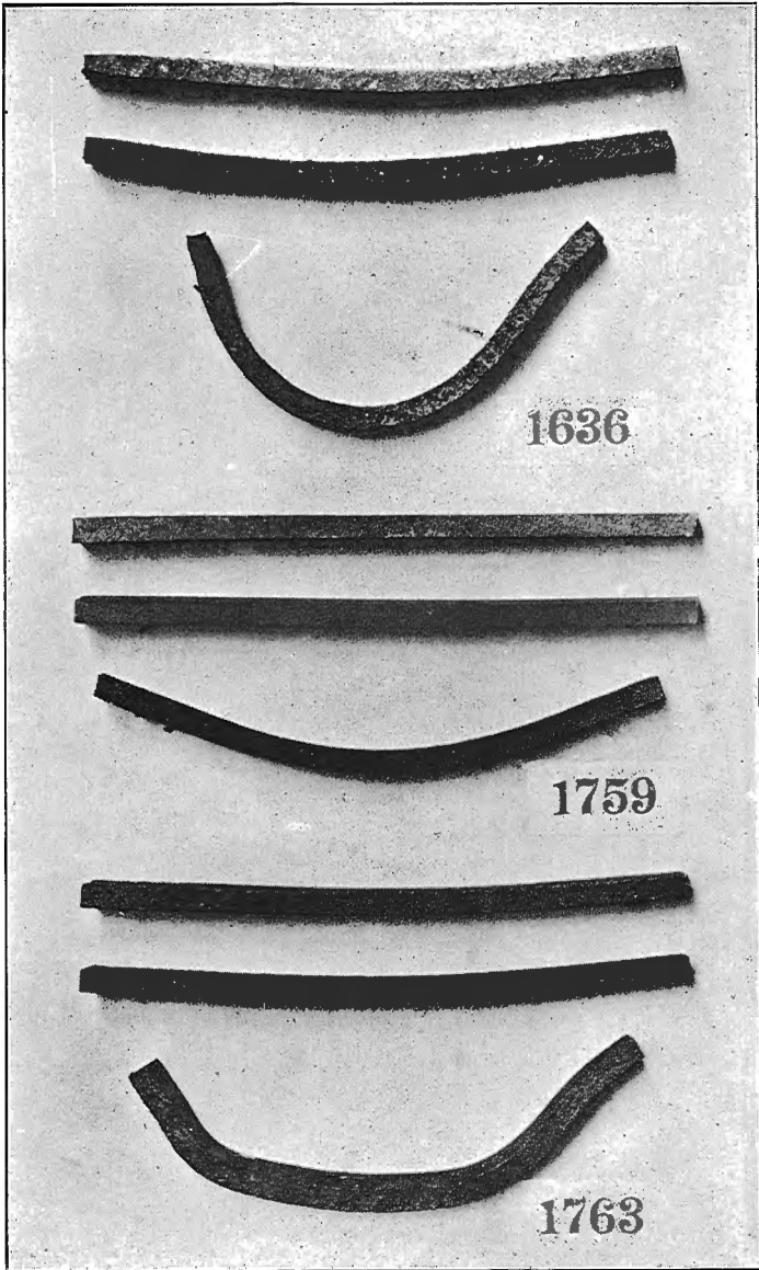
Strips of burned clay, used in the warpage test of roofing-tile clays.
