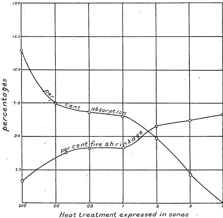
FIG. 3.—Absorption and fire shrinkage curves of clay 1807 from Dirt hills, Sask.
