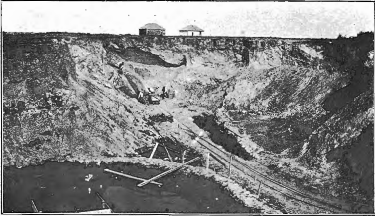
Clay pit at brick works, Saskatoon, Sask.
