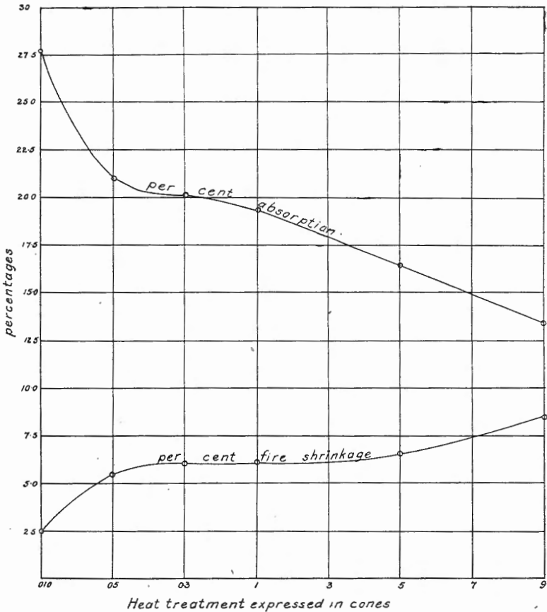
FIG. 1.—Absorption and fire shrinkage curves of shale from LaRivière, Man.
