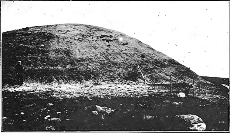
Knoll of brown sandy shale and soft sandstone, Dirt hills, Sask.
