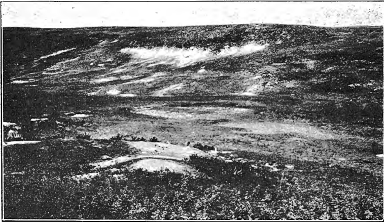
White sandy fireclay exposed in a coulee, Dirt hills, Sask.
