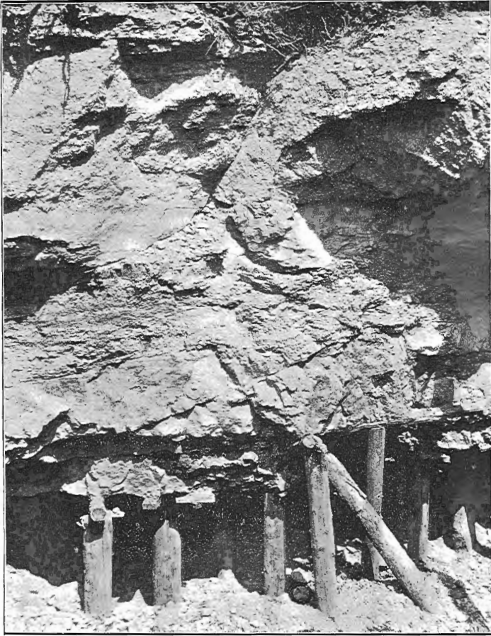
Section along railway of Clayburn Brick Co., Clayburn, B.C. The worked out bed of buff burning shale is overlain by sandstone and conglomerate,
