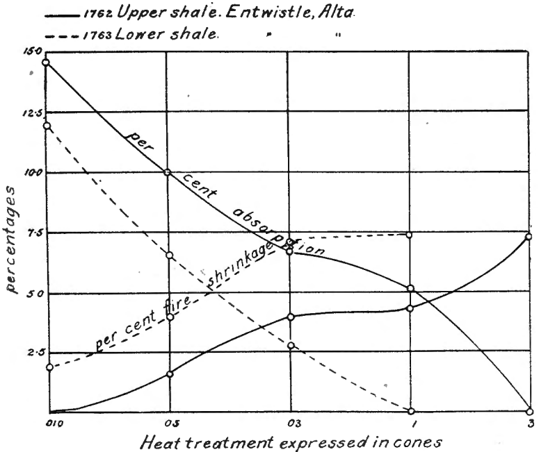
FIG. 4.—Absorption and fire shrinkage curves of shales from Entwistle, Alta.
