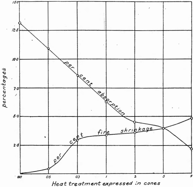
FIG. 5.—Absorption and fire shrinkage curves of sewer-pipe shale No. 1759, from Brickburn, Alta.
