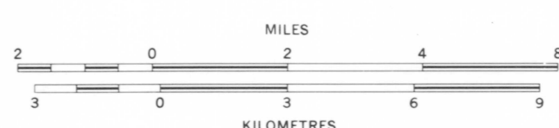
SURFICIAL GEOLOGY AND GEOMORPHOLOGY OF CAMSELL BEND 95J
